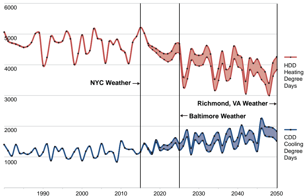
Fig. 11. Historical and Projected Number of Heating and Cooling Degree Days per Year for New York City (1980-2050)
