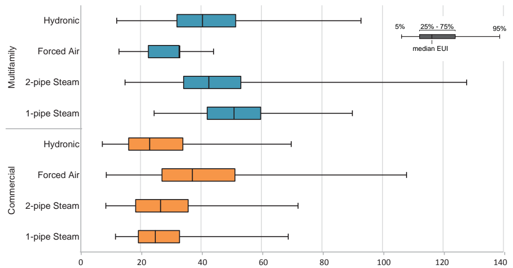
Fig. 17. Distribution of Heating EUIs by Heating Distribution Type in Multifamily Buildings (kBtu/SF)
