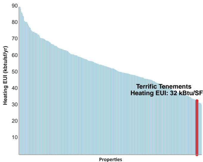
Heating EUIs in Building Typology: Multifamily, Pre-war, ≤ 7 Stories
