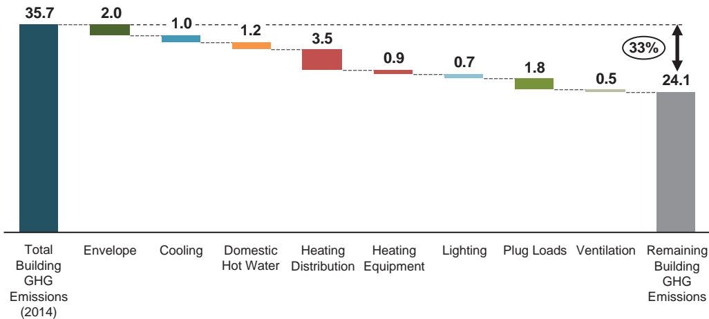
Fig. E5. GHG Reduction Potential of Identified ECMs (MtCO 2 e)
