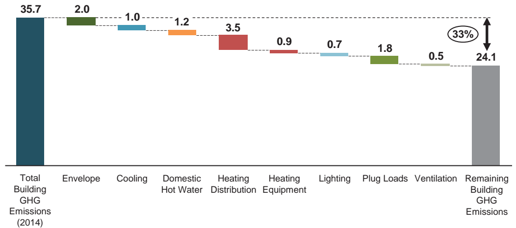
Fig. 24. Technical Potential for GHG Reductions from ECMs by Building System (MtCO 2 e)
