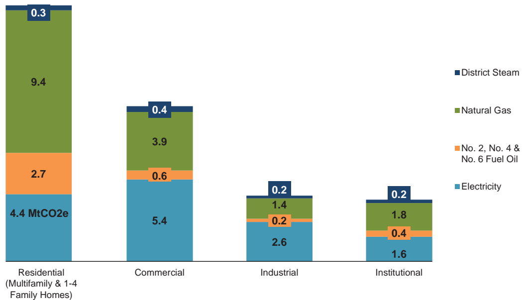
Fig. 14. GHG Emissions by Building Use and Fuel Types* in Million Metric Tons of Carbon Dioxide Equivalent (MtCO 2 e)
