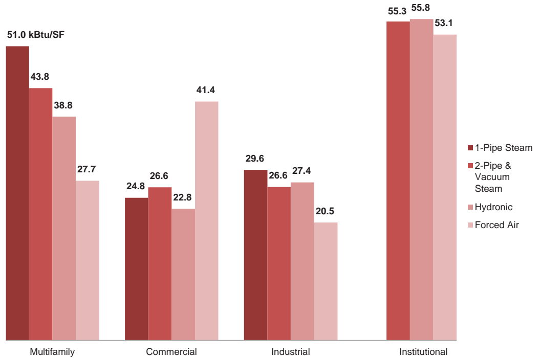
Fig. 18. Median Heating EUI by Heating Distribution System Type (kBtu/SF)
