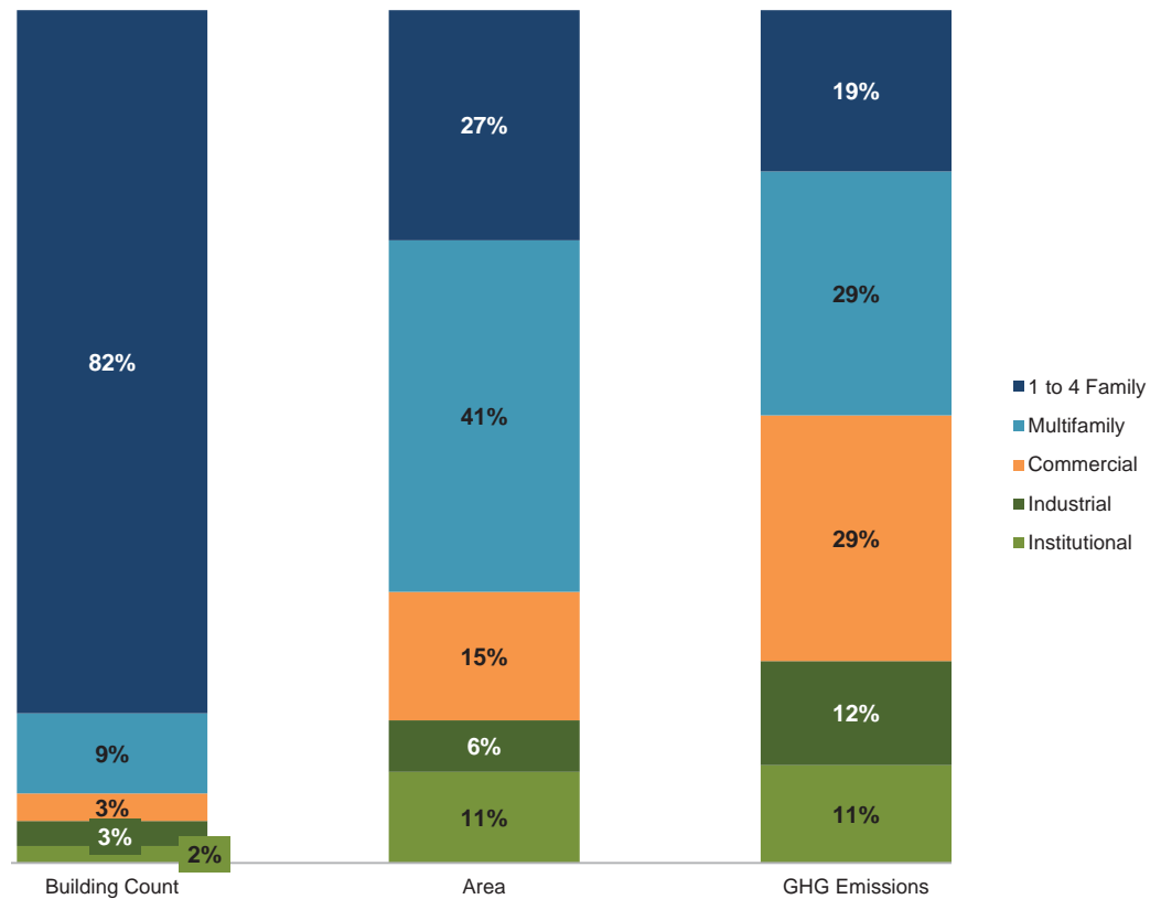
Fig. E3. Building Uses by Building Count, Floor Area, and GHG Emissions
