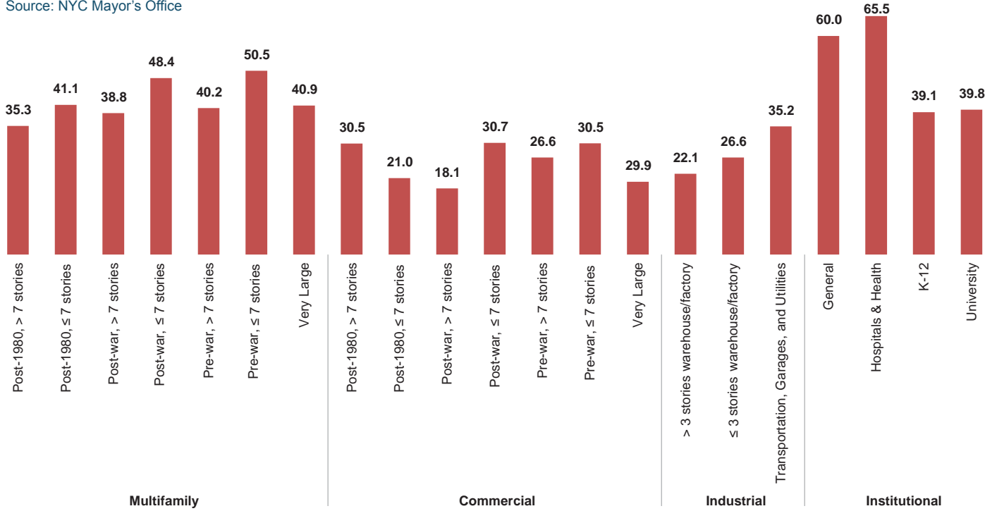
Fig. 20. Median Heating EUI by Building Typology (kBtu/SF)
