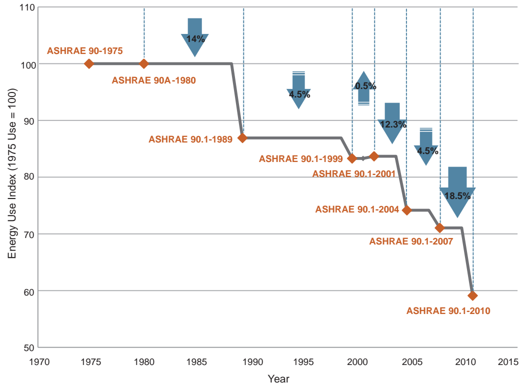
Fig. 32. ASHRAE 90.1 Energy Savings Advancements Since 1975
