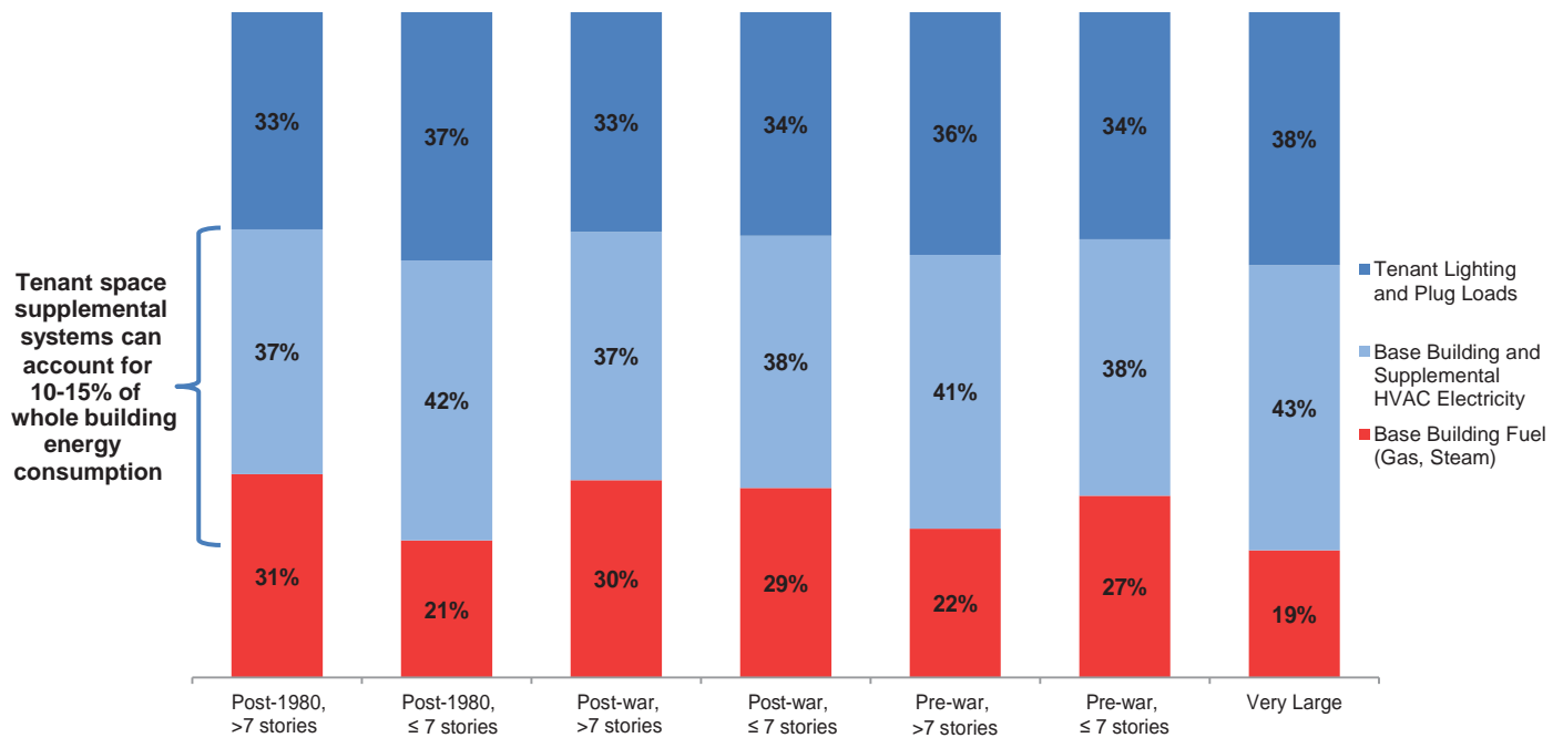
Fig. 38. Tenant Lighting, Tenant Plug Loads, and Base Building Energy in Commercial Buildings
