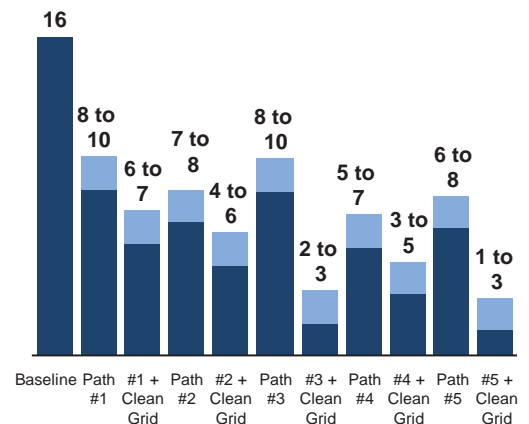
Path GHG Emissions Reduction (MtCO 2 e)
