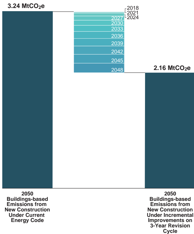
Fig. 33. Projected GHG Abated from New Construction Under Scenario of Replicating Historical Code Advancements
