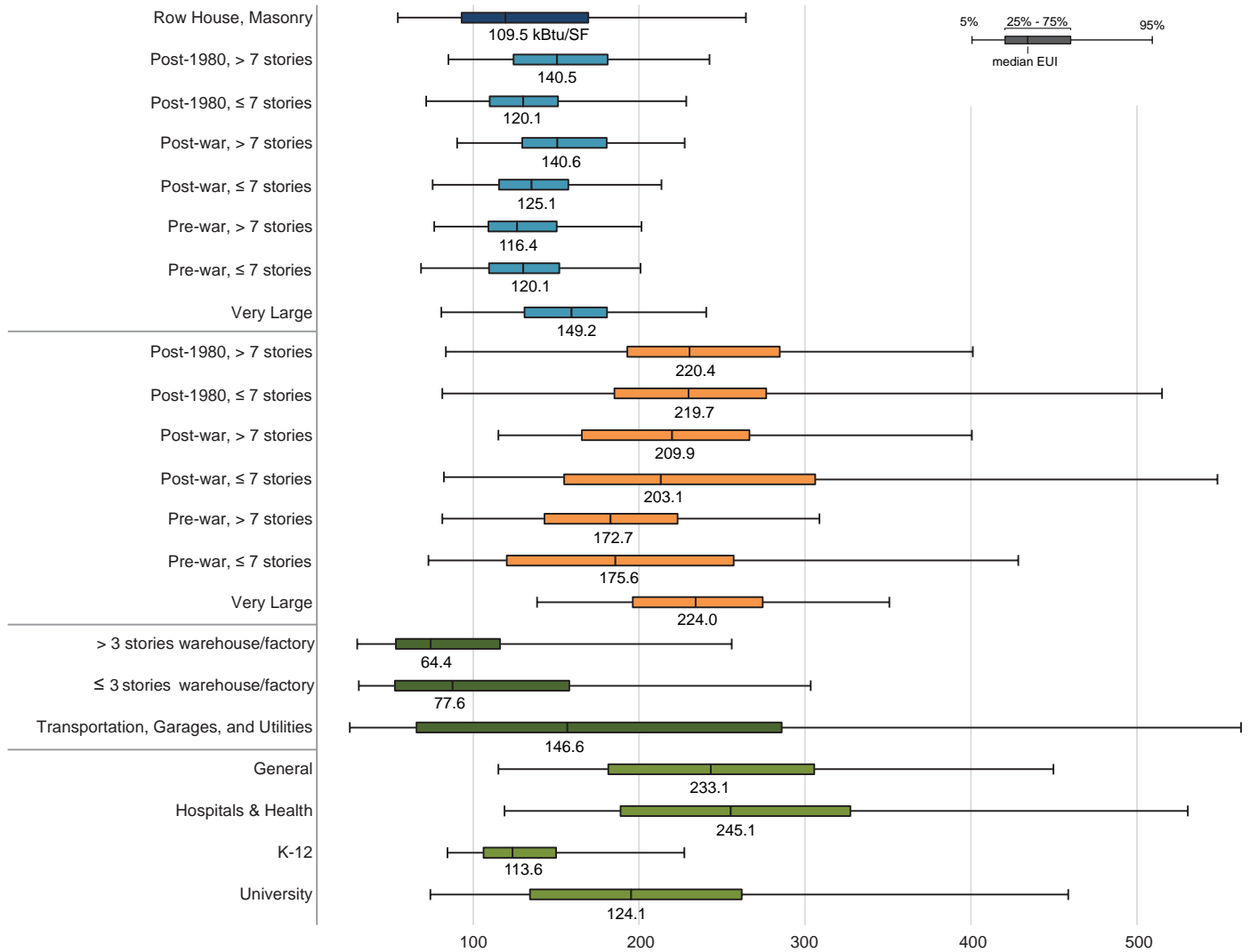
Fig. 8. Median and Distribution of Source EUI by Building Typology (kBtu/SF)
