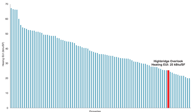
Heating EUIs in Building Typology: Multifamily, Post1980, >7 Stories
