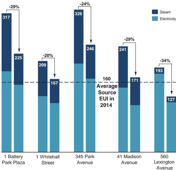
Whole Building Source EUI Reduction from RMC Commercial Portfolio (2005-2014)
