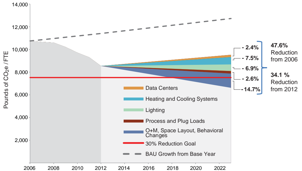
Fig. 29. NYC Carbon Challenge Completed and Projected ECMs
