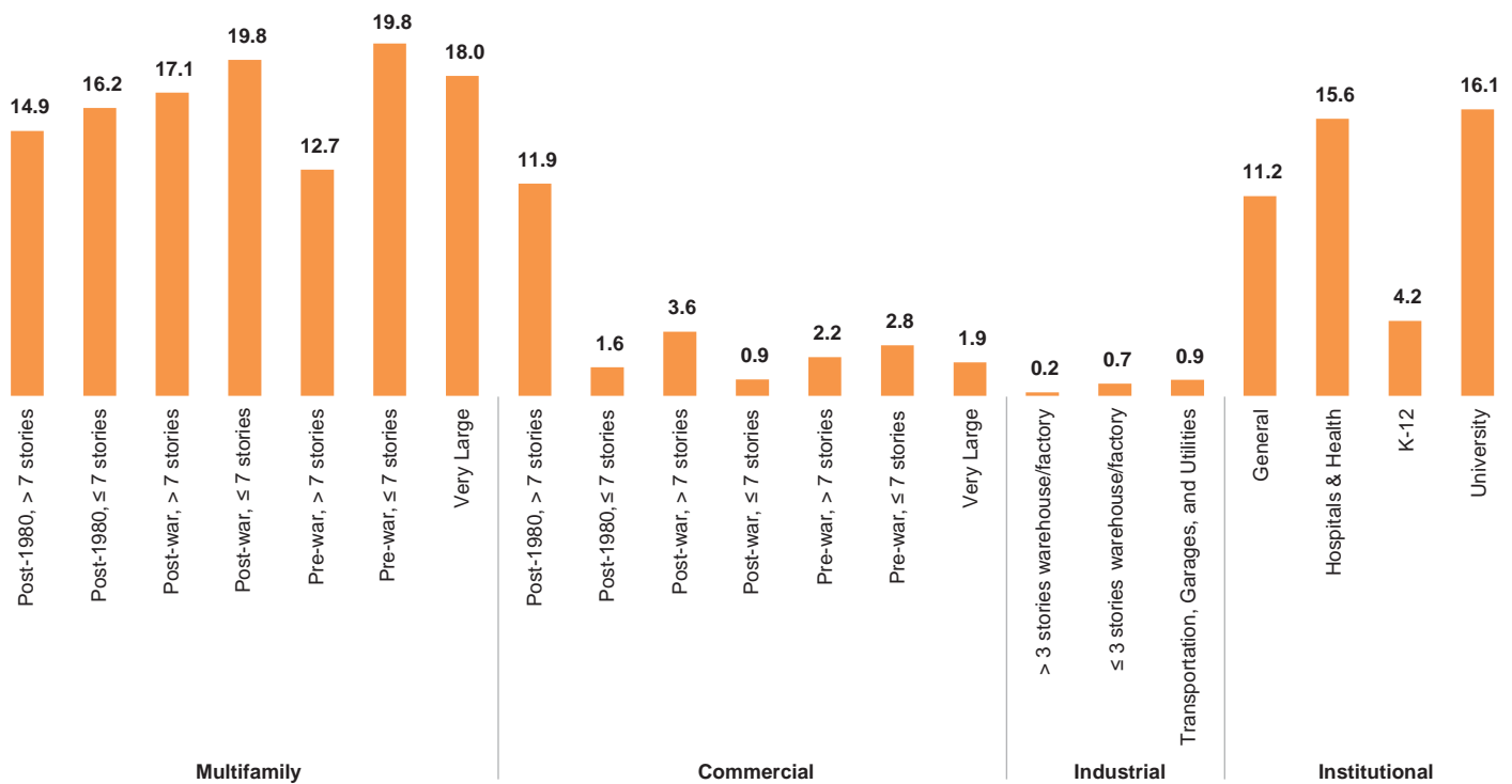
Fig. 21. Median Domestic Hot Water EUI by Building Typology (kBtu/SF)
