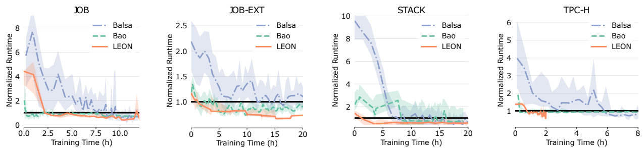
Figure 5: Training curves with variance on different datasets. The shaded area represents the range between the minimum and maximum values obtained from five different runs using different random seeds.
