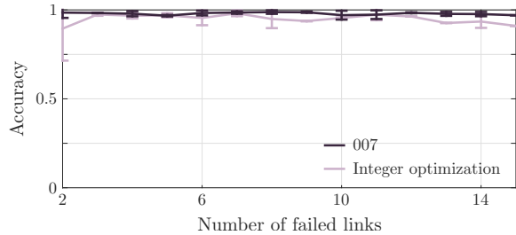
Figure 3: When Theorem 2 holds.
