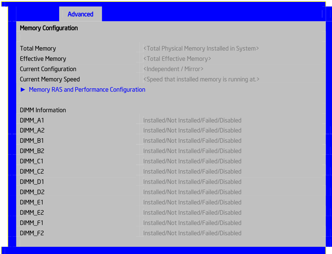
Figure 25. Setup Utility — Memory Configuration Screen Display
