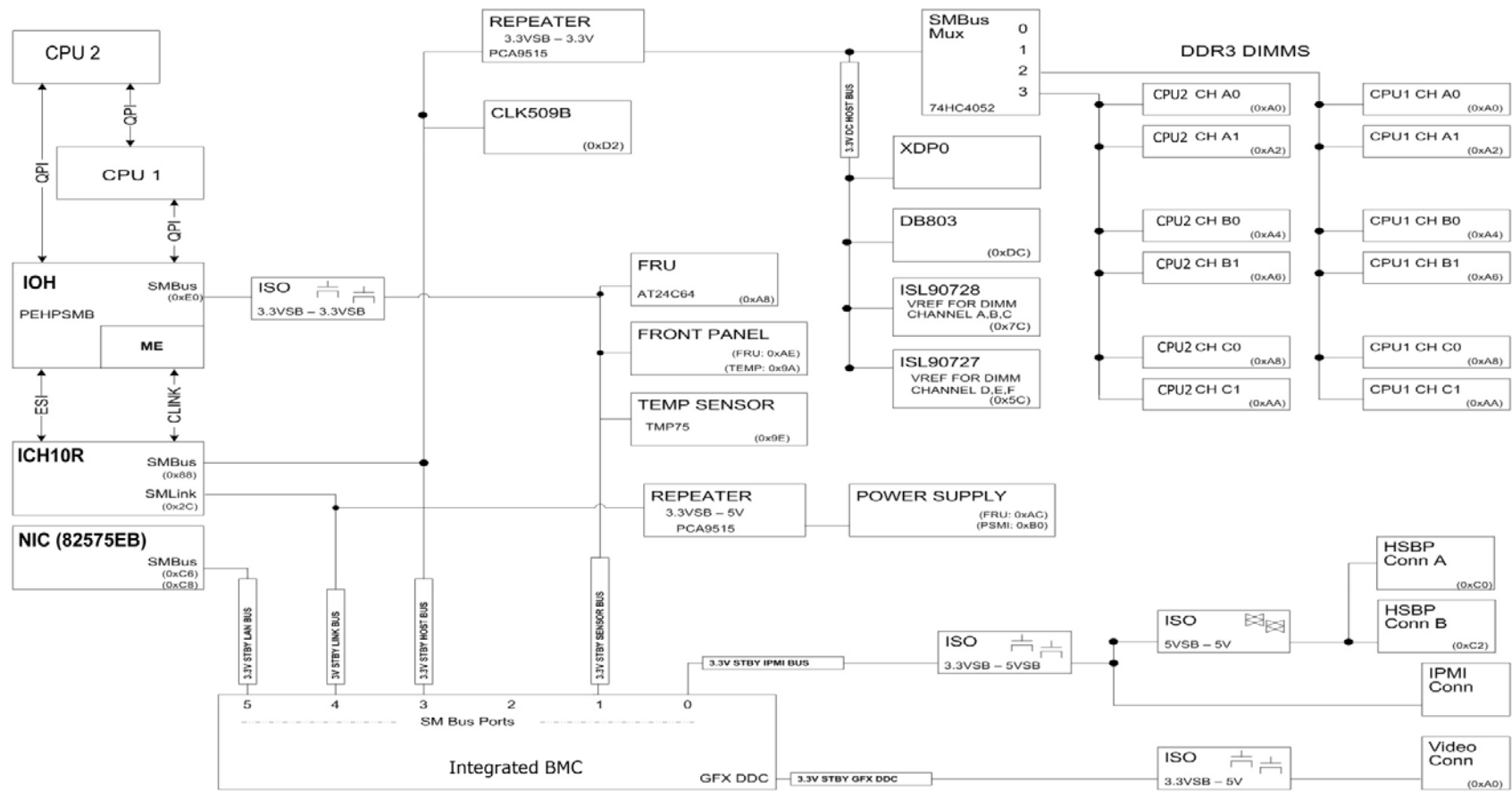
Figure 21. SMBUS Block Diagram
