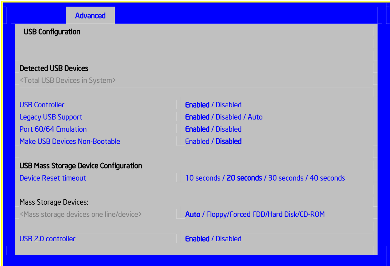
Figure 29. Setup Utility — USB Controller Configuration Screen Display
