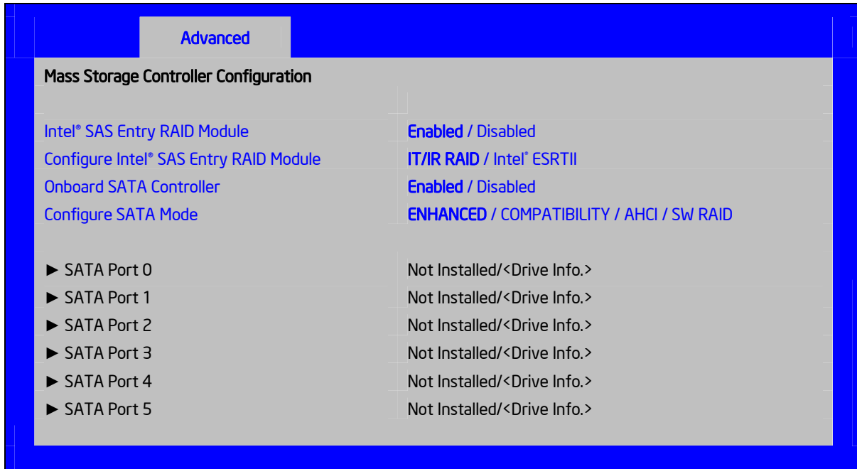
Figure 27. Setup Utility — Mass Storage Controller Configuration Screen Display
