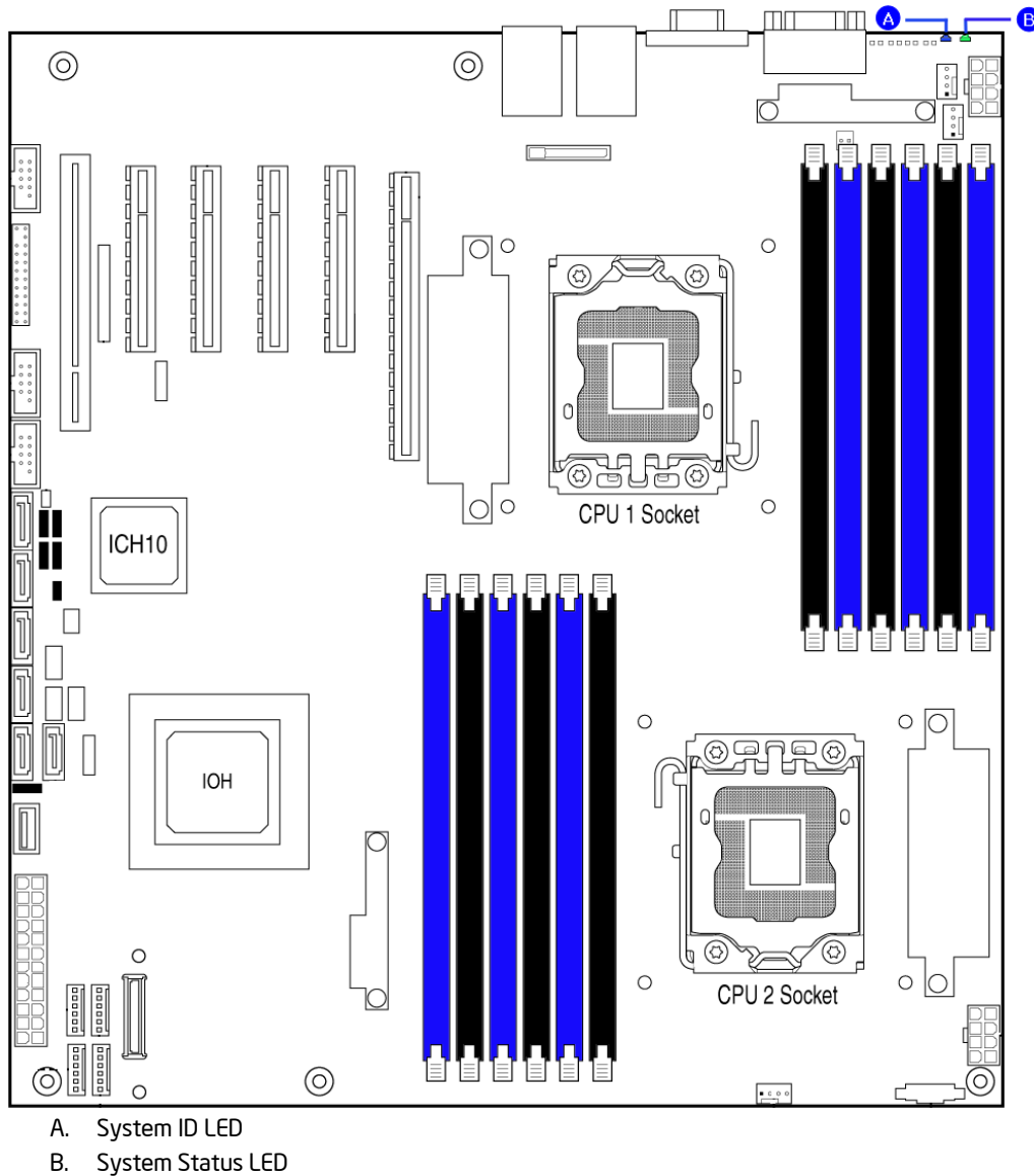
Figure 50. System Status LED Location
