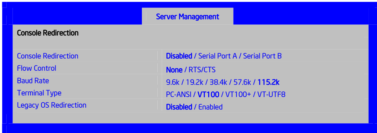
Figure 34. Setup Utility — Console Redirection Screen Display
