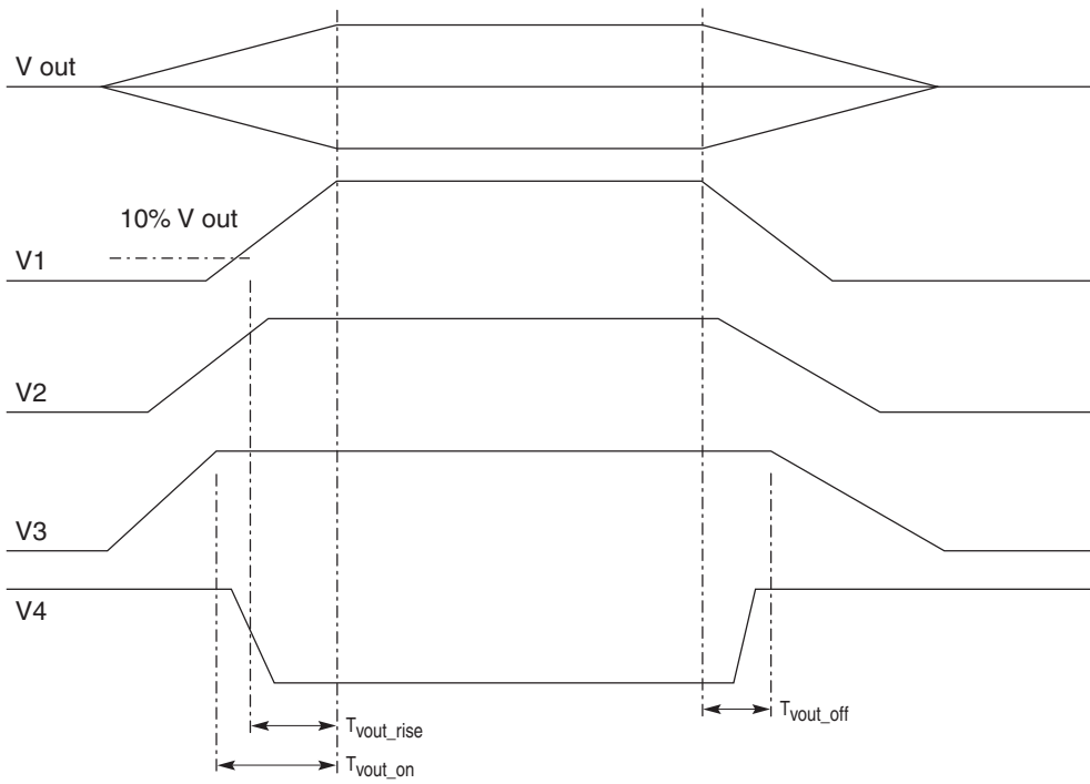
Figure 54. Output Voltage Timing
