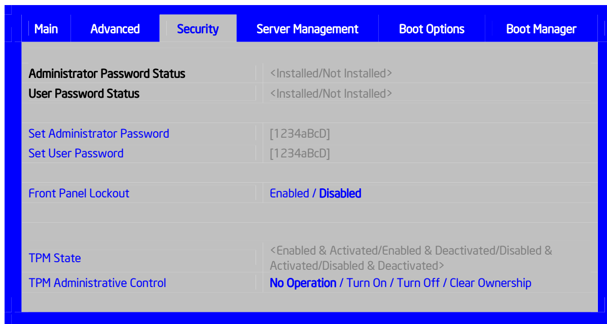
Figure 32. Setup Utility — Security Configuration Screen Display
