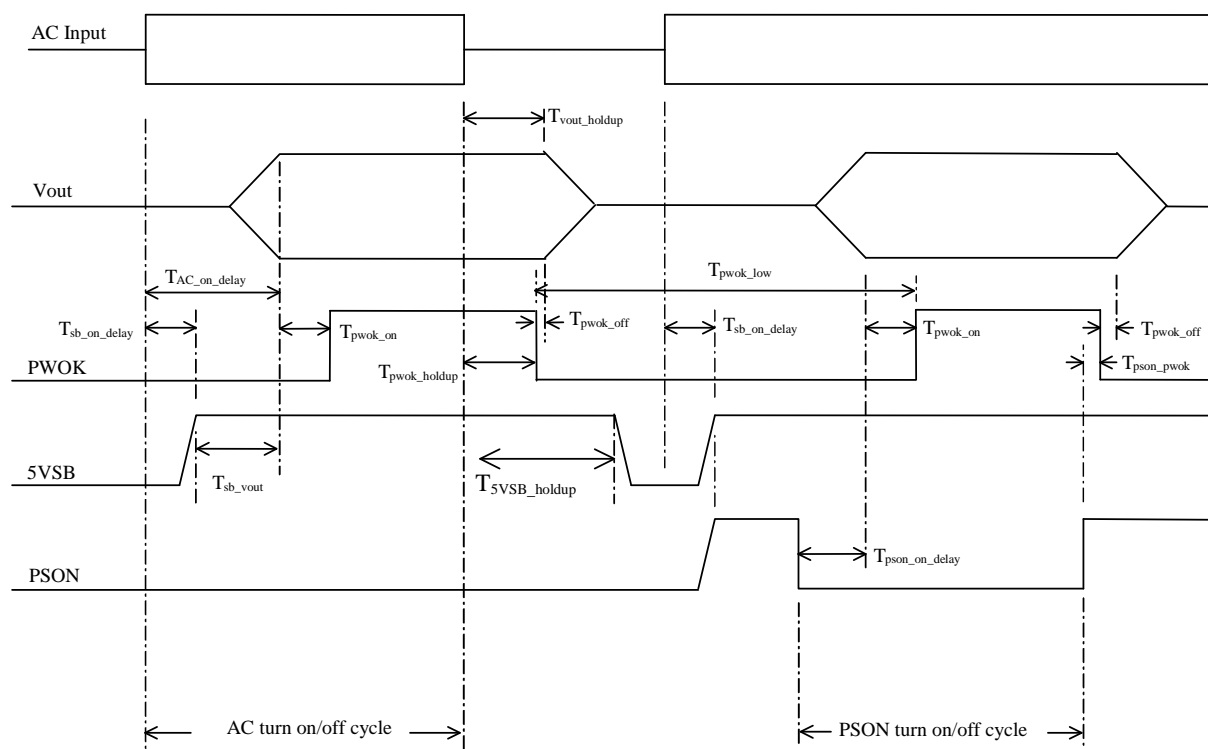
Figure 55. Turn On/Off Timing (Power Supply Signals)
