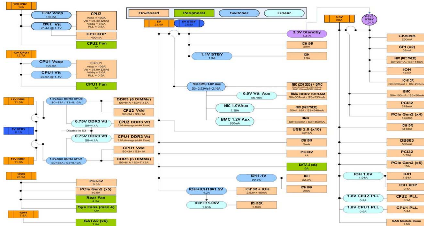
Figure 53. Power Distribution Block Diagram
