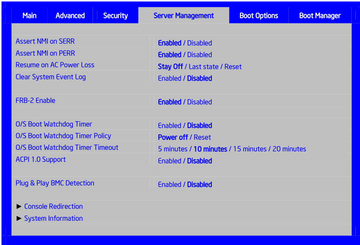
Figure 33. Setup Utility — Server Management Configuration Screen Display
