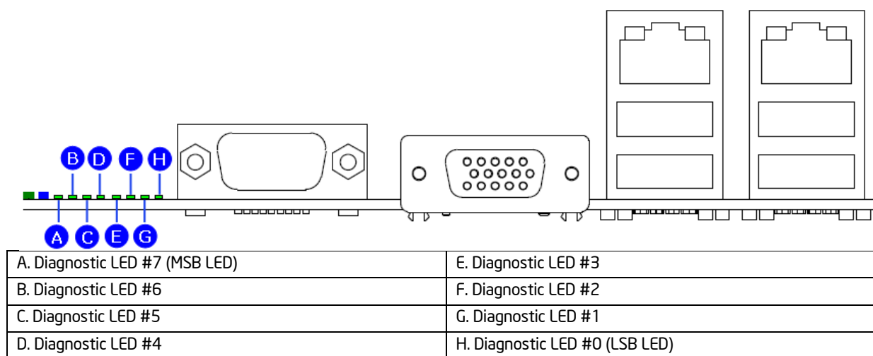
Figure 57. Diagnostic LED Placement Diagram
