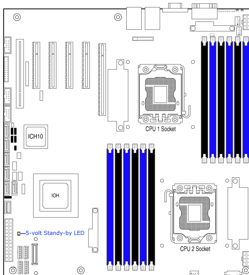
Figure 48. 5-volt Stand-by Status LED Location
