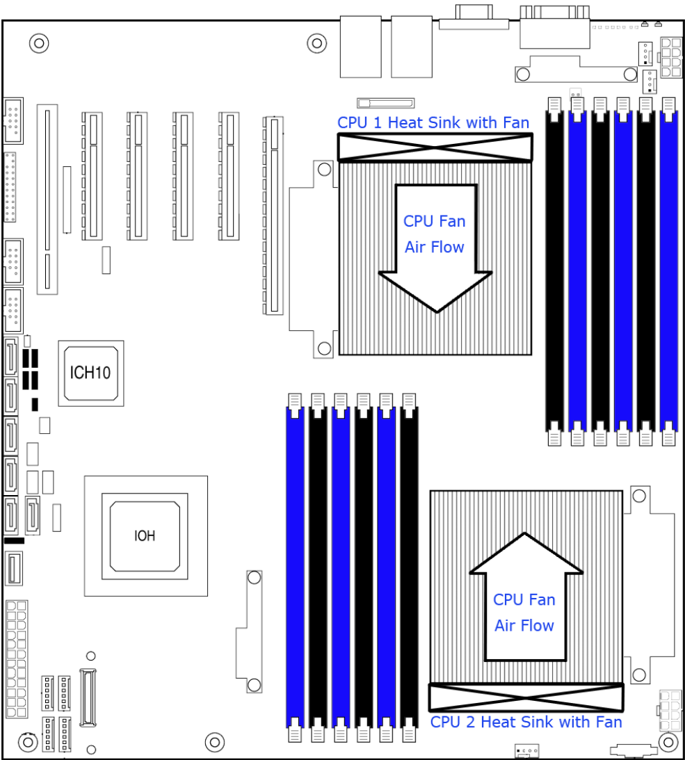
Figure 56. Active Processor Heatsink Installation Requirement
