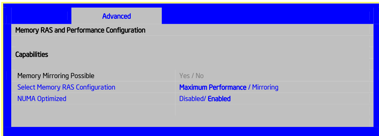
Figure 26. Setup Utility — Configure RAS and Performance Screen Display
