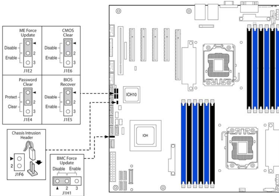
Figure 47. Jumper Blocks (J1E2, J1E4, J1E5, J1E6, J1H1)
