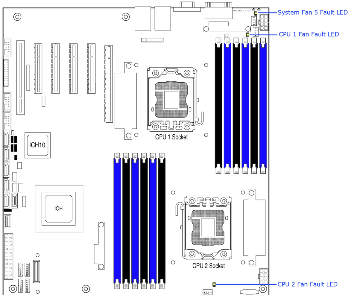
Figure 49. Fan Fault LED's Location
