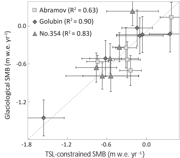
Figure 9. Comparison of modelled annual SMB constrained by TSL observations and glaciological SMB for Abramov, Golubin and Glacier no. 354. Uncertainties in the annual SMB are indicated.
