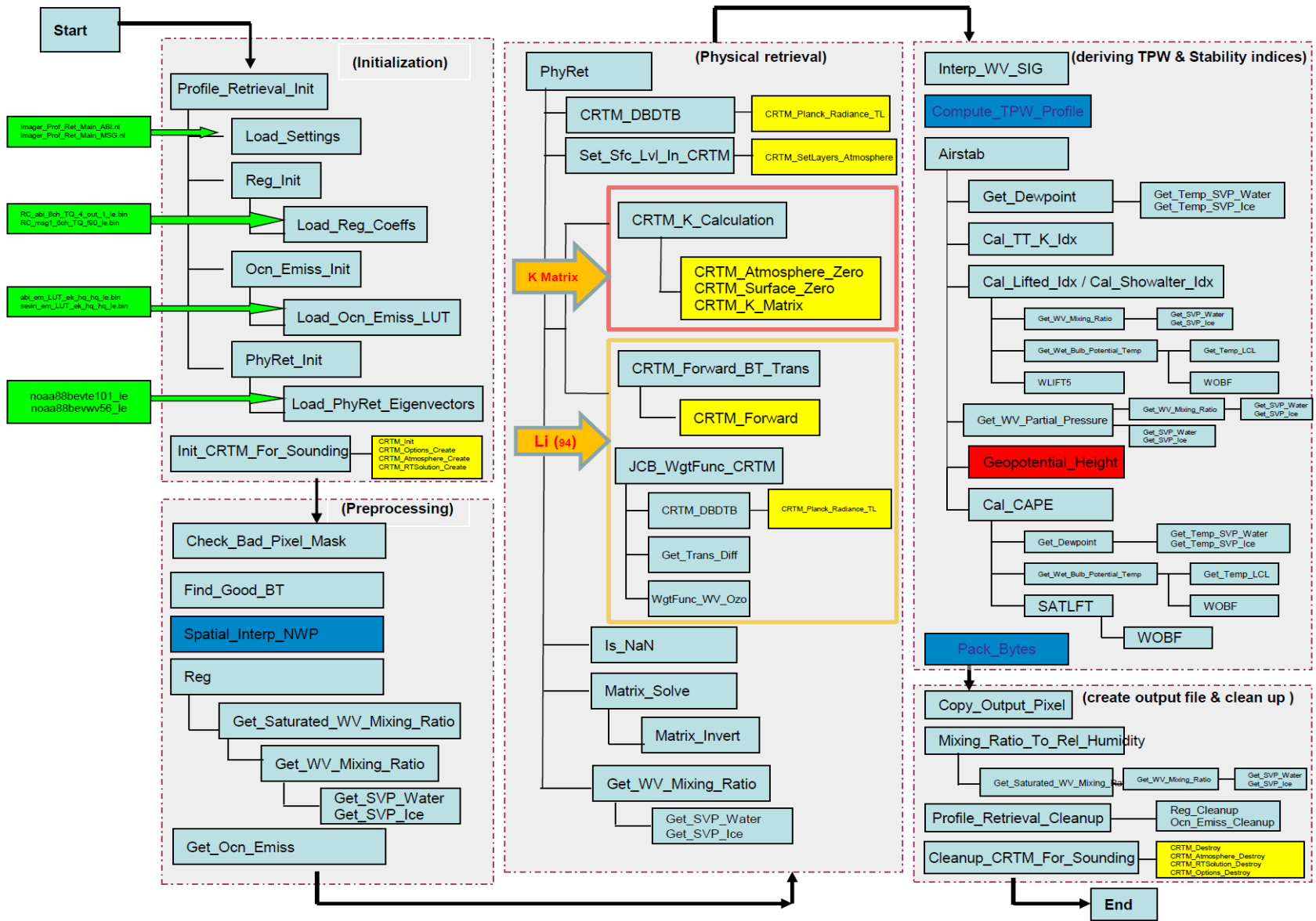
Fig A1: The sketch map of all ancillary inputs and routines applied in the LAP sounding algorithm. External routines are shown in colored boxes: CRTM (yellow), the Profile Utility library (red), or routines described in the GOES_R AIADD (blue). Profile Utility is available here: ftp://ftp.emc.ncep.noaa.gov/jcsda/CRTM/ancillary/
