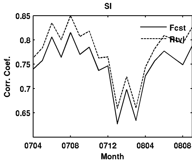
Figure 47. Same as Figure 32 but for SI.
