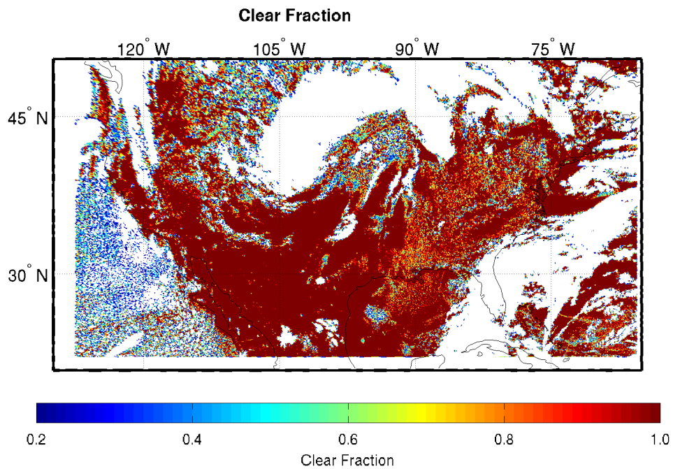
Figure 15: Clear sky fraction ( = Num_Clr_Pix / Block_Size**2) using a simulated ABI case; FORs with fraction lower than 0.2 are not retrieved.
