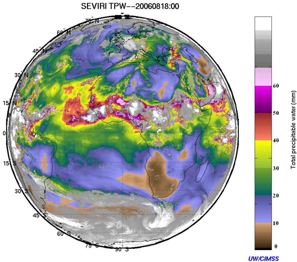
Figure 26. Example of LAP TPW from 00 UTC August 18, 2006 produced from SEVIRI on MET-8.
