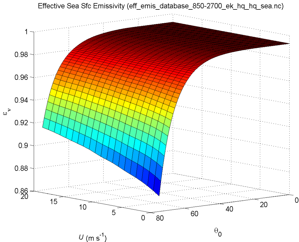
Figure 14: Sea surface emissivity ( \varepsilon_v ) against LZA ( \theta_0 ) and wind speed ( U ).
