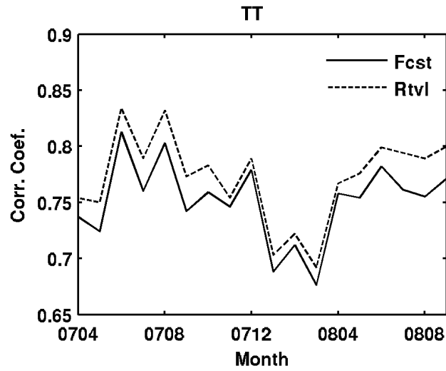
Figure 45. Same as Figure 32 but for TT.
