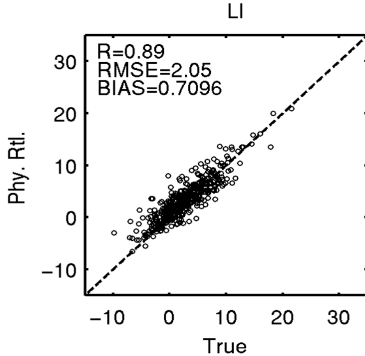
Figure 33. Same as Figure 28 but for Lifted Index. Radiosondes are used as truth. The monthly averaged time series of LI between April 2007 and September 2008 over Europe and North Africa is plotted in the following. The difference between forecast and retrieval is trivial because temperature profile and low-level moisture profile have very little improvement.
