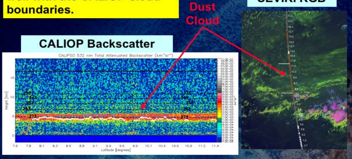
Figure 14: The GOES-R volcanic ash retrieval algorithm was applied to an elevated Saharan dust cloud, which exhibits a spectral signature that is very similar to ash in the infrared. The results of the height retrieval algorithm are overlaid (white circles) on a 532 nm CALIOP total attenuated backscatter cross section. The retrieval results agree well with the lidar positioning of the dust cloud.
