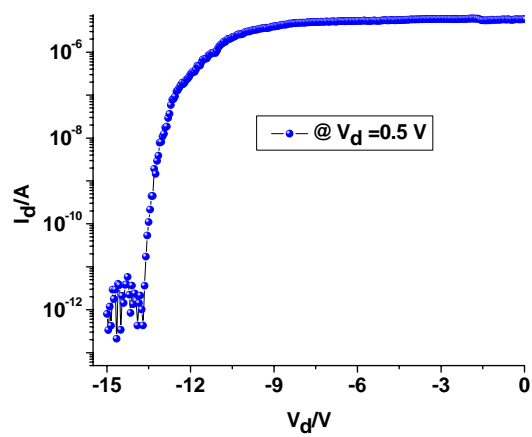
S1- I_d - V_g characteristic of the OCD at a constant V_d of 0.5 V.
