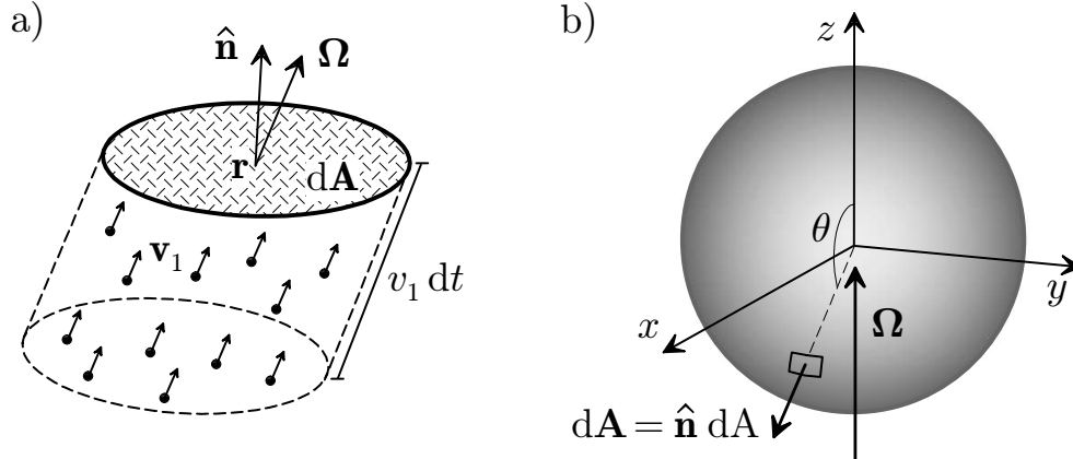
Figure 5.1: Surfaces in a radiation field. a) A surface element d\mathbf{A} in a field of particles moving with the same velocity \mathbf{v}_1 . In a time interval dt the surface element is crossed by the particles that initially are within the volume that would be swept by the surface if it were moving with velocity -\mathbf{v}_1 . b) Schematic diagram of the coordinate system used to calculate the integral of Eq. (5.8) over the surface of the sphere.
