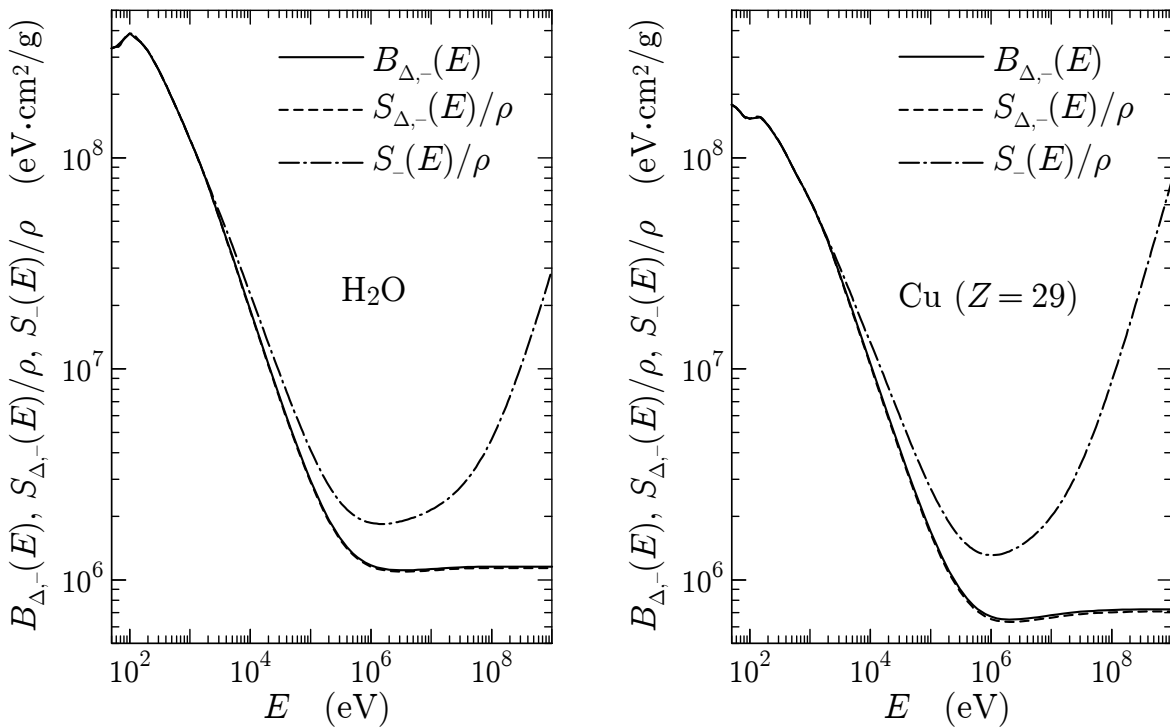
Figure 5.2: Mass energy absorption, B_{\Delta,-}(E) , restricted mass stopping power, S_{\Delta,-}(E)/\rho , and mass stopping power, S_{-}(E)/\rho , of electrons in water and copper, calculated with \Delta_{-} = \Delta_{+} = 1 keV and \Delta_{\gamma} = 0 . For projectiles with energies less than about 10 keV, the MEA practically coincides with the restricted mass stopping power.
