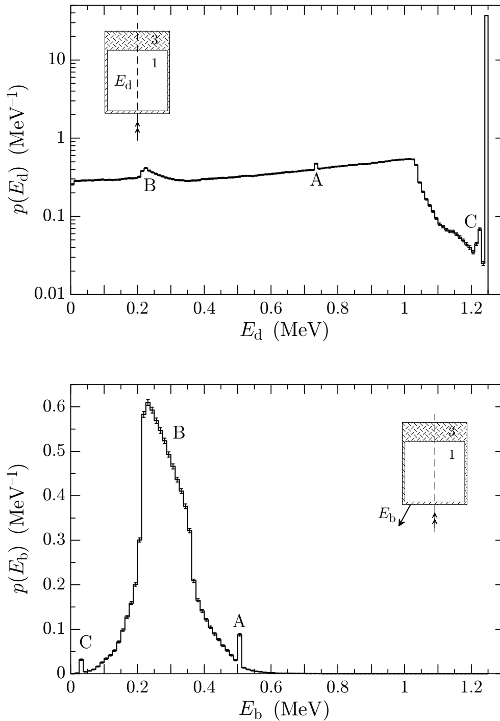
Figure 7.4: Partial results from pencyl for the NaI photon detector described in the text (input file cyld.in ). Top: distribution of energy deposited in the NaI crystal (MAT=1). Bottom: energy distribution of backscattered (downbound) photons.
