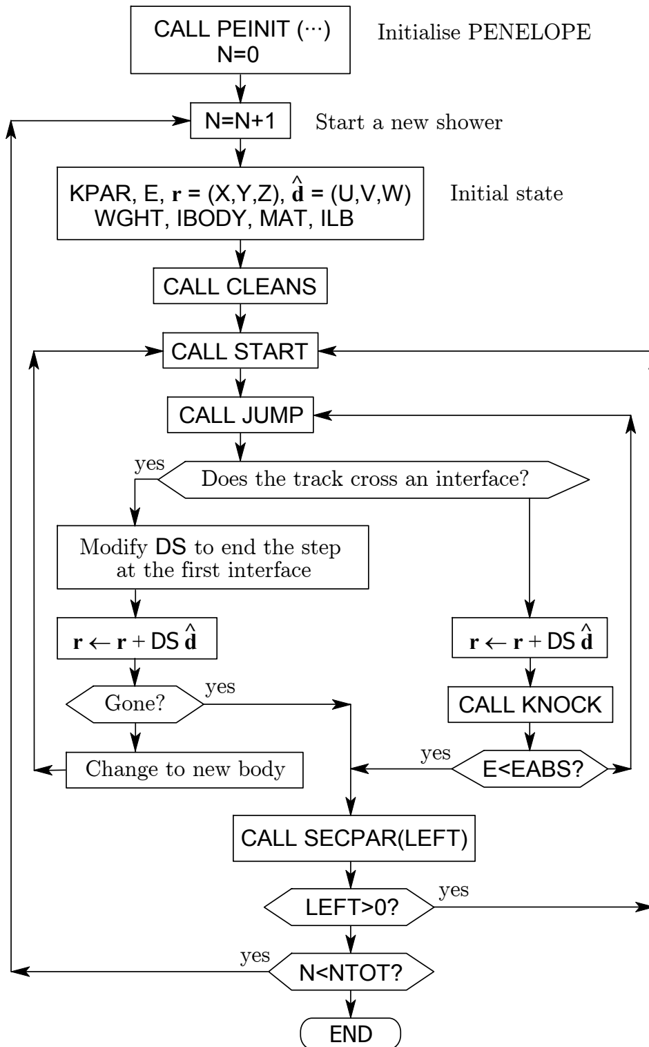
Figure 7.1: Flow diagram of the main program for simulating electron-photon showers with PENELOPE.
