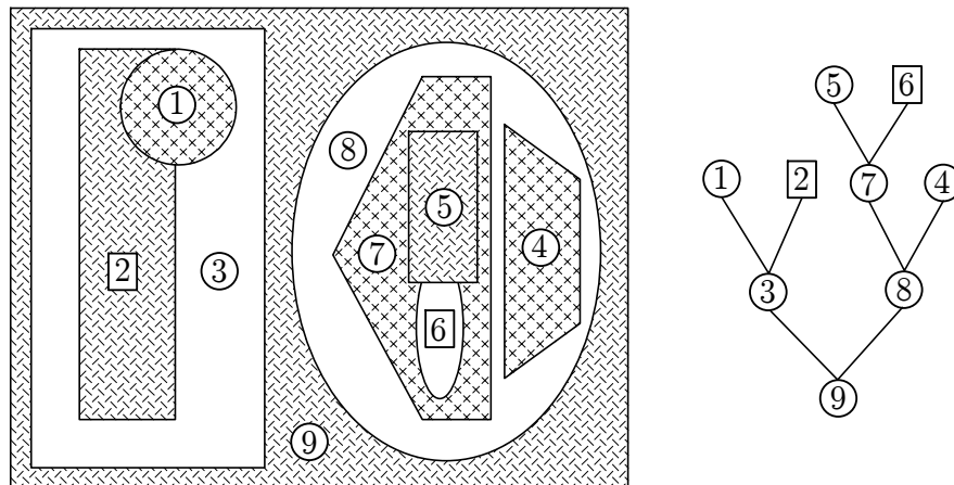
Figure 6.6: Planar cut of a geometry example, showing modules (number labels in circles) and bodies (number labels in squares), and the associated genealogical tree. Notice that a module can always be defined as a body limited by their submodules and daughter bodies, but this affects the structure of the genealogical tree and, therefore, the efficiency (speed) of the geometry operations.
