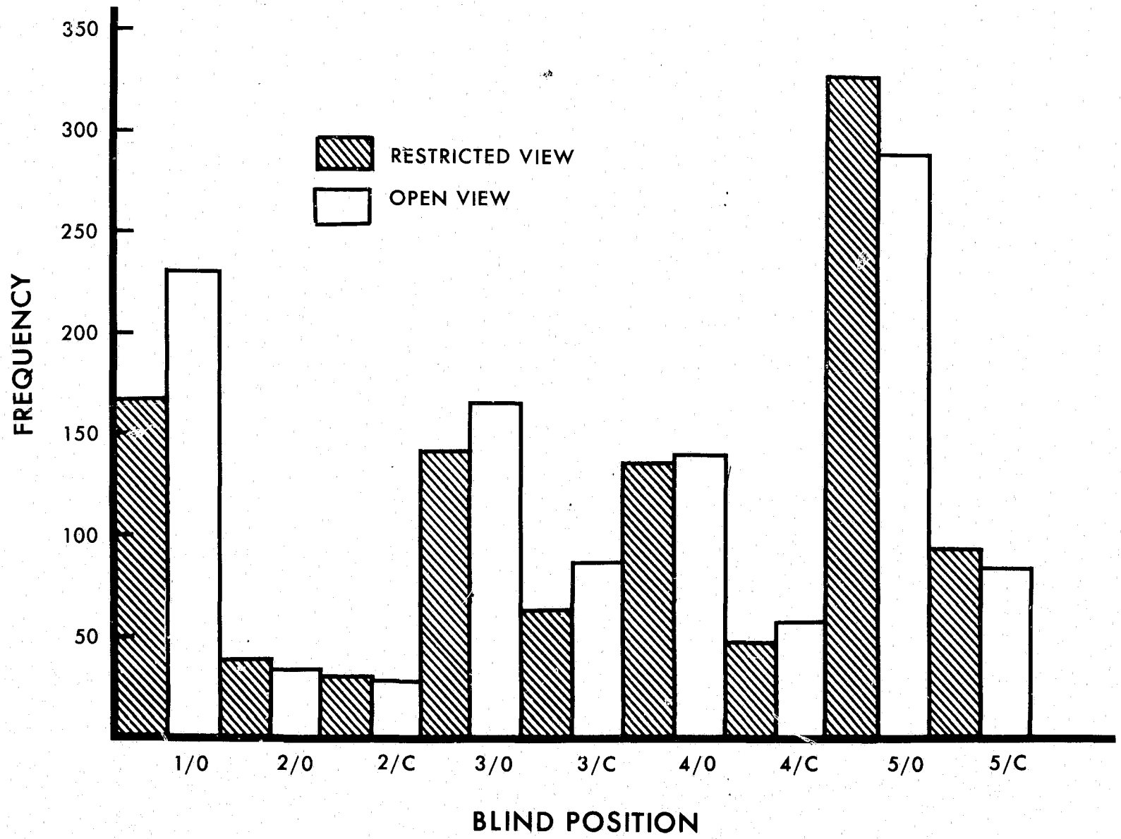
FIGURE 13. DISTRIBUTION OF BLIND POSITIONS BY VIEW BEFORE TREATMENT.
