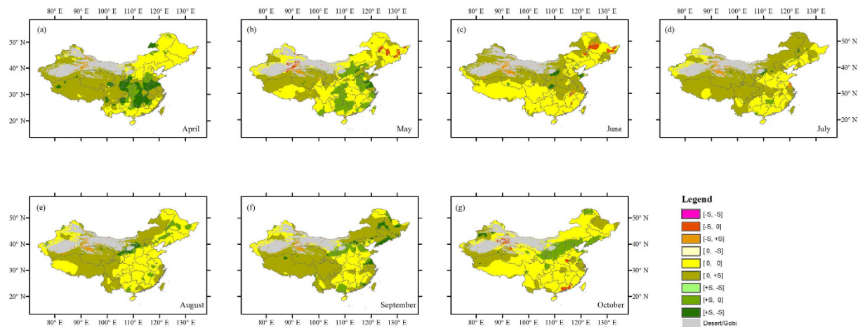
Figure 2. Comparison of trends of NDVI and temperature for April–October (a–g). Statistically significant (the absolute value of MK test equal to or greater than 1.96) positive trends are denoted as +S, negative trends as –S and insignificant ones as 0. The first character in each pair right the color bar denotes NDVI trend and the second one denotes temperature trend. This figure was generated using ArcGIS 10.1 ( http://www.esri.com/software/arcgis/ ).
