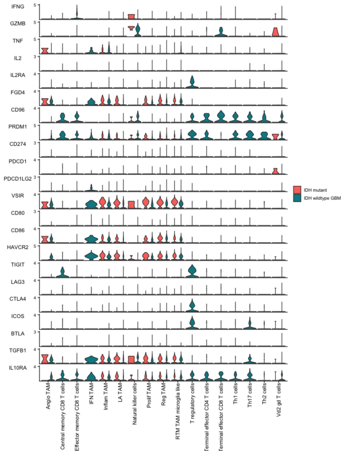
Figure 7. Violin plot of gene expression values in TAMs and T cells between GBM and IDH-mutant glioma.
