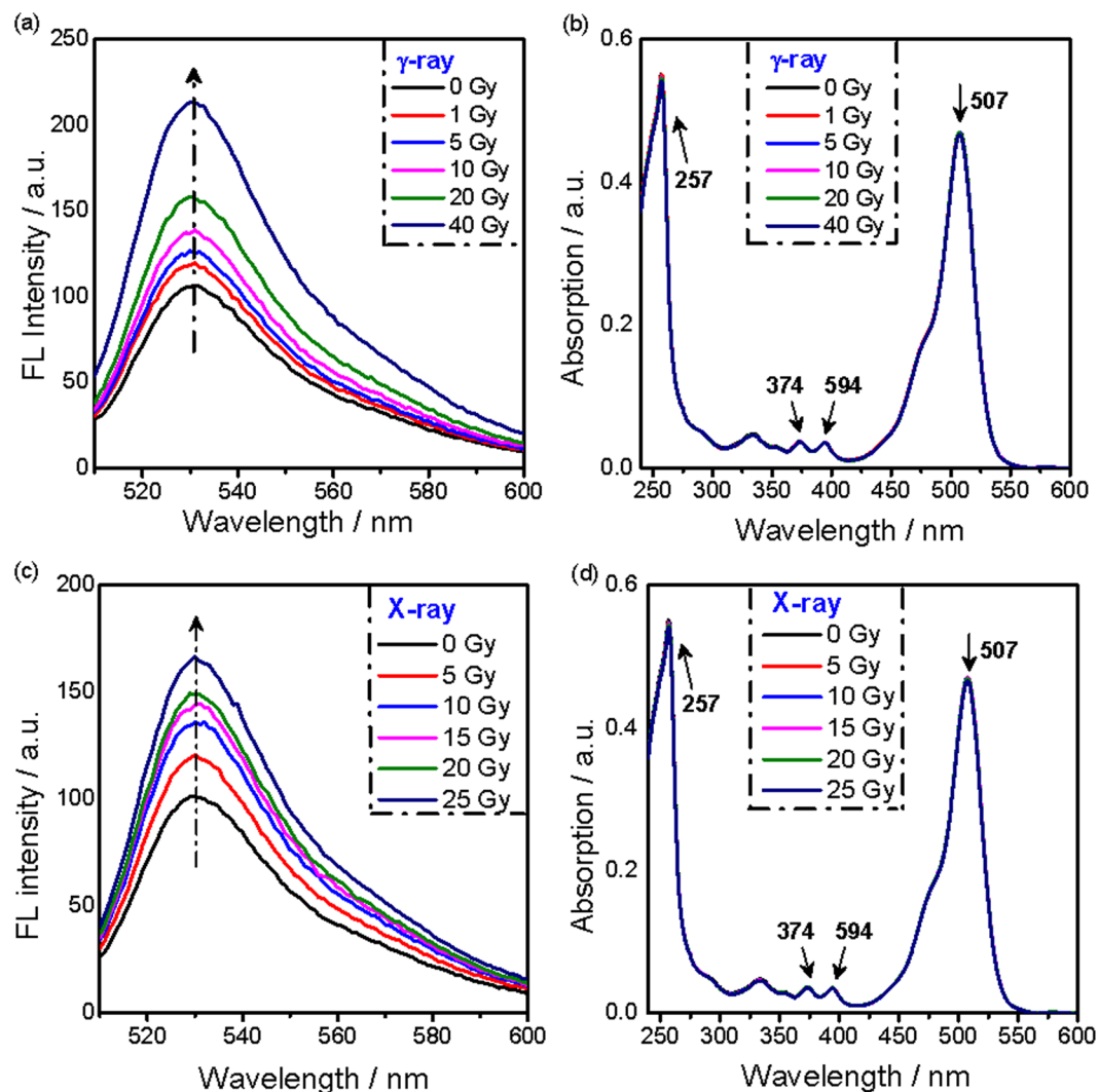
Figure 2. (a) Fluorescence spectra of SOSG solutions (5 \mu\text{M} ) for varied radiation doses delivered by a ^{60}\text{Co} source ( \lambda_{\text{ex}} = 504 \text{ nm} ); (b) UV-vis absorption spectra of SOSG solutions (5 \mu\text{M} ) for different radiation doses delivered by a ^{60}\text{Co} source; (c) Fluorescence spectra of SOSG solutions (5 \mu\text{M} ) for different X-ray doses; (d) UV-vis absorption spectra of the SOSG solution (5 \mu\text{M} ) for different X-ray doses.
