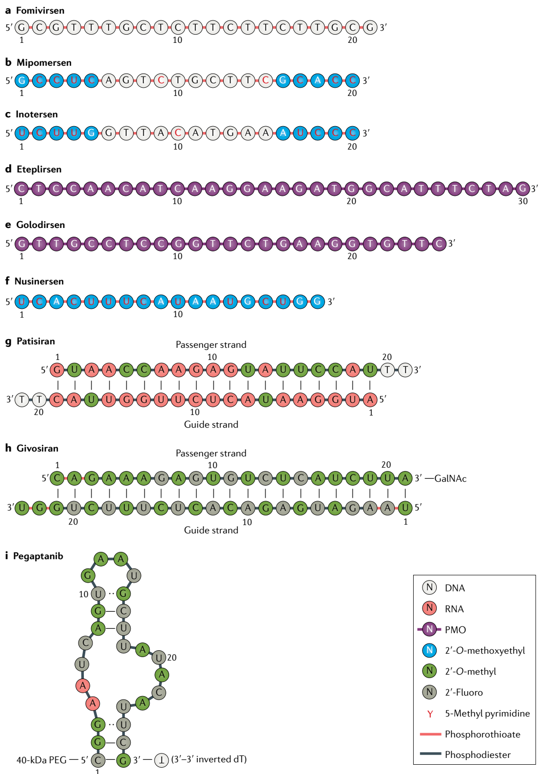
Fig. 1 | Chemistry of FDA-approved oligonucleotide drugs. Chemical composition of the FDA-approved oligonucleotide drugs fomivirsen (part a), mipomersen (part b), inotersen (part c), eteplirsen (part d), golodirsen (part e), nusinersen (part f), patisiran (part g), givosiran (part h) and pegaptanib (part i). Drugs are ordered by mechanism of action. Drug names, trade names, principal developing company, modality and RNA target are described in TABLE 1 for each compound. The drug defibrotide consists of a mixture of single-stranded and double-stranded ribonucleotides of variable length and sequence composition harvested from pig intestine. It therefore cannot be easily represented in the same manner as the other oligonucleotide drugs and so is not shown here. GalNAc, N-acetylgalactosamine; PEG, polyethylene glycol; PMO, phosphordiamidate morpholino oligonucleotide. Part i structure adapted from REF. 284 , Springer Nature Limited.
