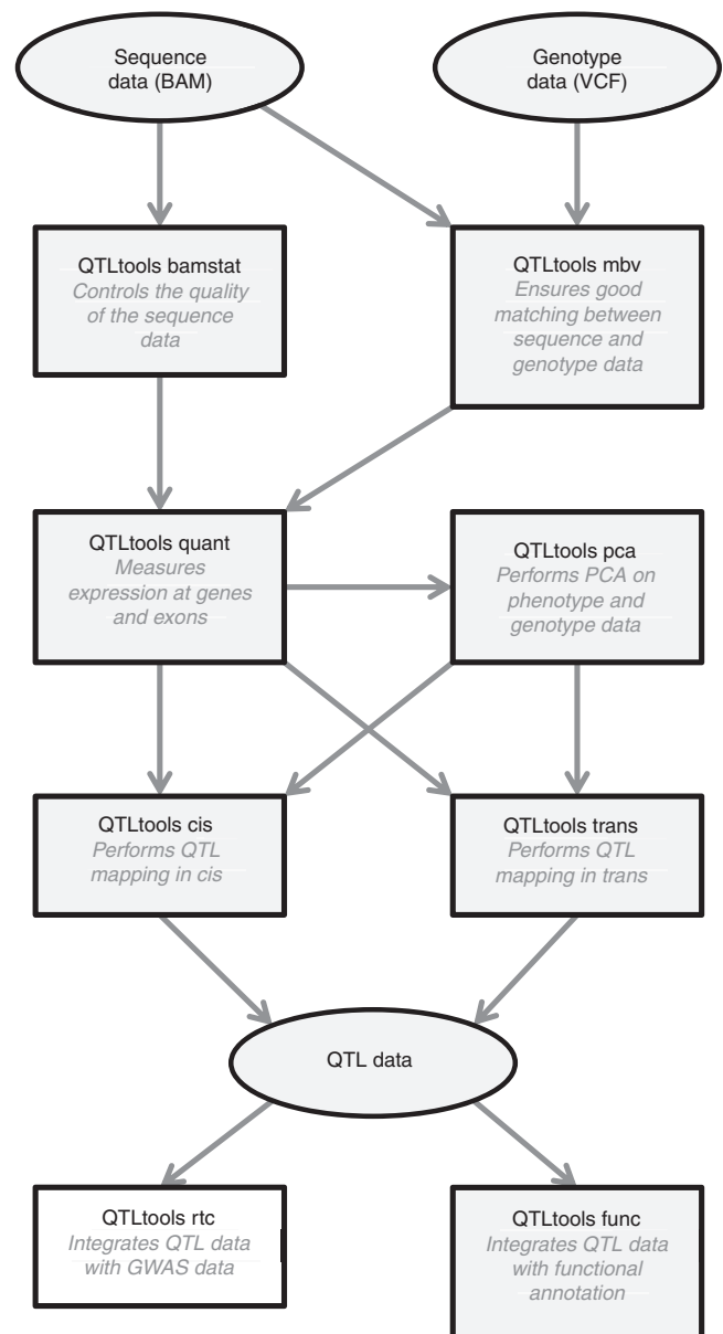
Figure 1 | Flow chart of the main QTLtools functionalities. This represents how the various functionalities of QTLtools can be combined to go from the raw sequence and genotype data to collections of molecular QTLs which can then be integrated with both GWAS data and functional annotations. Data is represented with ovals and tasks with boxes in which the name of the mode is shown in bold black with a short description of what it does.
