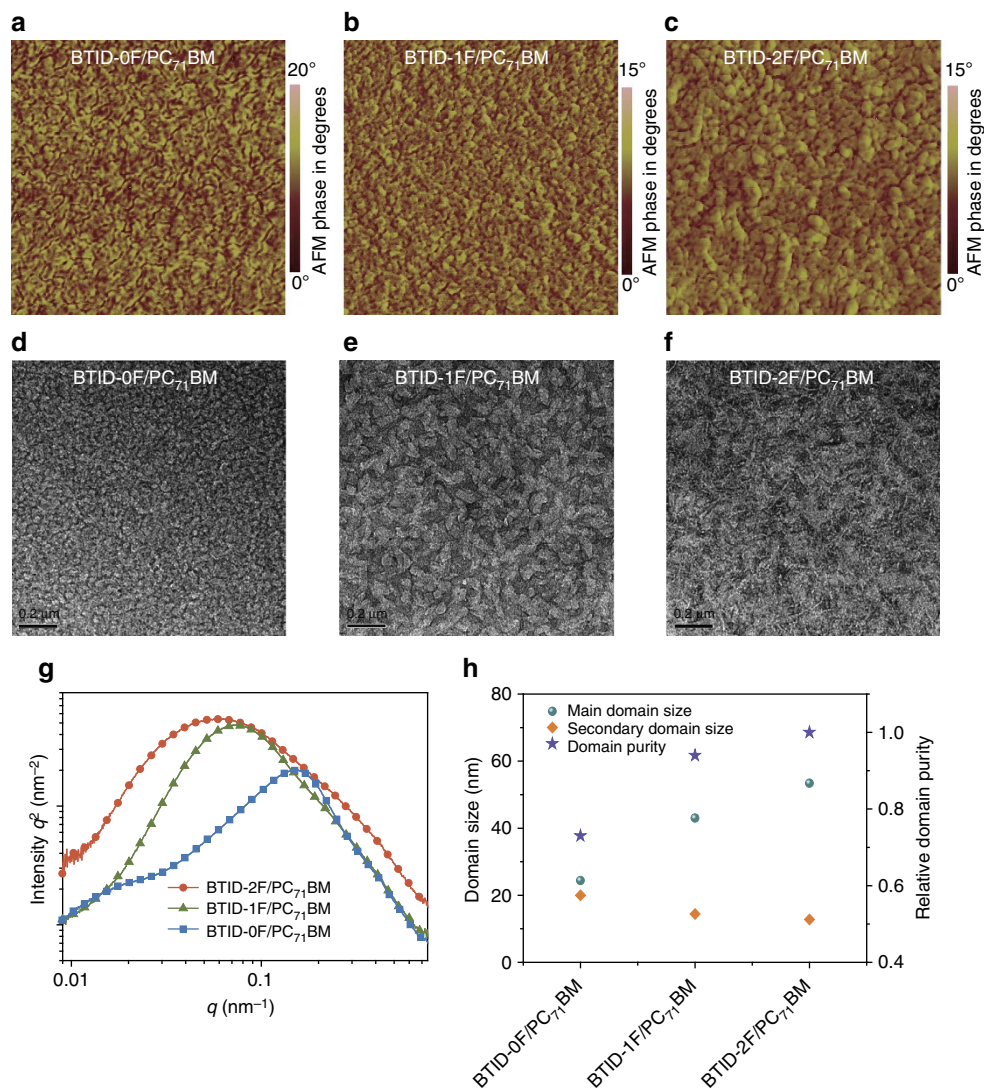
Figure 4 | Lateral morphologies and microstructures of blend films on ZnO/ITO substrates. (a–c) AFM phase images; (d–f) TEM images; (g) RSoXs profiles; and (h) relative domain purity and domain sizes.
