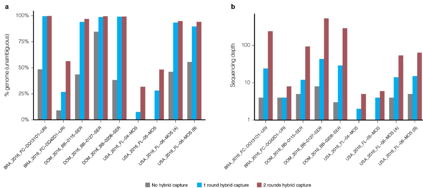
Extended Data Figure 6 | Evaluating multiple rounds of Zika virus hybrid capture. Genome assembly statistics of samples before hybrid capture (grey), and after one (blue) or two (red) rounds of hybrid capture. Nine individual libraries (eight unique samples) were sequenced all three ways, had more than one million raw reads in each method, and
