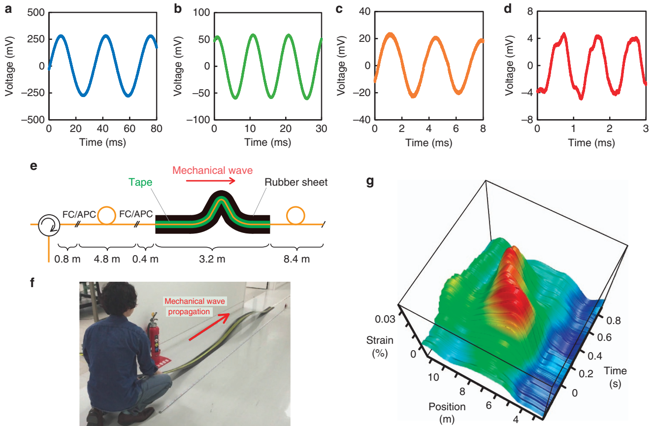
Figure 9 Ultrahigh-speed measurement results. Temporal variations (deviation from the initial value) of the output DC voltage when dynamic strains were applied to a 0.4-m-long section at (a) 30 Hz, (b) 100 Hz, (c) 300 Hz and (d) 1 kHz. (e) Schematic structure and (f) photograph of the FUT while tracking the propagation of a mechanical wave. (g) Measured temporal variation of the strain distribution.
