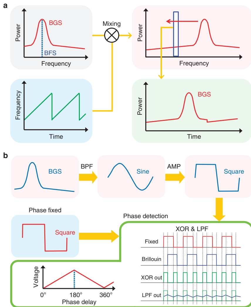
Figure 2 Principles of high-speed acquisition of BGS and BFS. (a) BGS acquisition. By mixing with a frequency-swept microwave, the BGS originally observed in the frequency domain can be obtained in the time domain at high speed. (b) BFS acquisition. The BGS is approximated by a one-period sinusoidal waveform and rectified. Its phase delay, which corresponds to the BFS, is then detected using an XOR logic gate and an LPF. The output voltage is in one-to-one correspondence with the phase delay in the range from 0 to 180^\circ .
