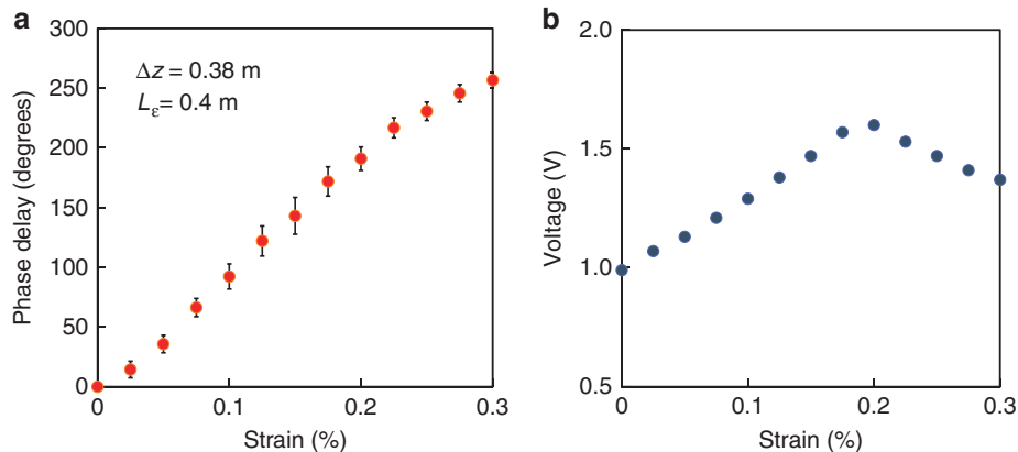
Figure 7 Phase delay and output DC voltage measured as functions of applied strain. (a) Strain dependence of the phase delay. The spatial resolution \Delta z was 0.38 m, and the length of the strained section L_e was 0.4 m. Averaging was performed 10 times. The error bars were calculated at each strain as the standard deviations of 100 data plots. The slope in the range from 0 to 0.20% was 952 degrees/%. (b) Strain dependence of the output DC voltage. The slope in the range from 0 to 0.20% was 3.2 V/%.
