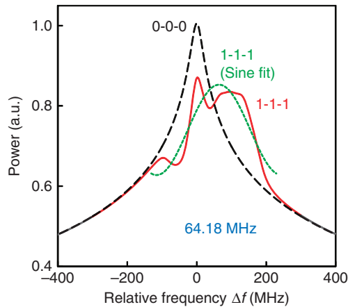
Figure 8 Example of the simulated BGSs. The black dashed curve is the simulated BGS for the FUT configuration '0-0-0' (refer to Supplementary Fig. S2 for the definition), and the red solid curve is that for '1-1-1'. The green dotted curve, which is the sinusoidal fit of the solid curve, becomes maximal at \Delta f = 64.18 MHz.
