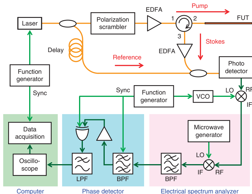
Figure 1 Configuration of ultrahigh-speed BOCDR. Experimental setup. EDFA, erbium-doped fibre amplifier; IF, intermediate frequency; LO, local oscillator; RF, radio frequency.
