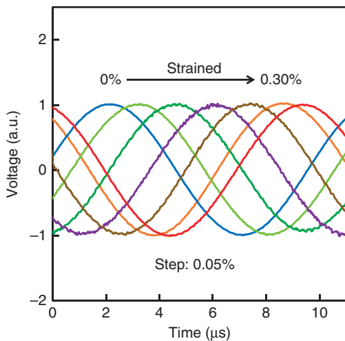
Figure 6 Strain dependence of the normalised BGS approximated by a one-period sinusoidal waveform. The spatial resolution \Delta z was 0.38 m, and the length of the strained section L_e was 0.4 m. Averaging was performed 10 times.
