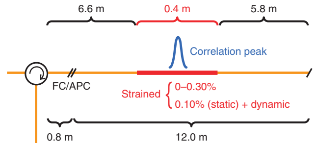
Figure 4 Structures of FUT. Strains of up to 0.30% were applied to a 0.4-m-long section of a 12.8-m-long silica SMF, which was composed of a 0.8-m-long pigtail of an optical circulator connected to a 12-m-long SMF using an FC/APC adaptor.
