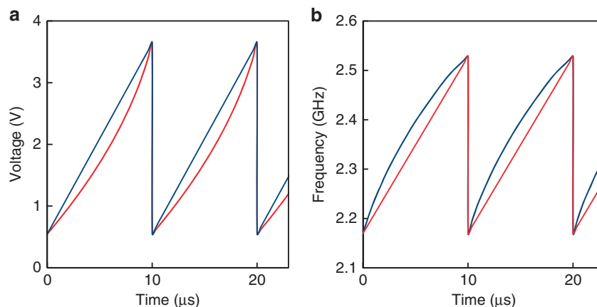
Figure 3 VCO operation with a BFS sampling rate of 100 kHz. (a) Linearly applied voltage (blue) and pre-distorted applied voltage (red). (b) Output frequencies when the voltage was applied in linear (blue) and pre-distorted (red) manners.
