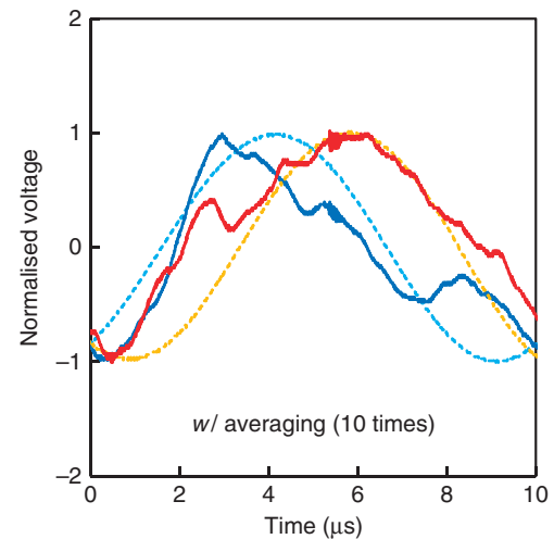
Figure 5 Normalised raw and sinusoidally approximated BGSs. The red and blue solid curves indicate the raw BGSs with and without 0.07% strain, respectively; whereas the orange and aqua dashed curves are the approximated BGSs with and without 0.07% strain, respectively. Averaging was performed 10 times.
