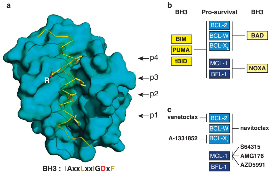
Figure 2 Interaction of BCL-2 family members. (a) The canonical BH3/surface groove interaction in the family. Structure of BCL-X L (blue surface representation) bound to the amphipathic helical BH3 peptide of BIM (a yellow ribbon indicates its helical structure) 27 (PDB/3FDL), with its N terminus at the bottom. Underneath the protein is a consensus BH3 sequence of the pro-apoptotic proteins (x denotes nonconserved residues). The four key hydrophobic amino acids (yellow) of the BIM BH3 peptide that bind to pockets p1 to p4 in BCL-X L are highlighted, as is the invariant aspartic acid (D) (oxygens in red) that binds to a conserved arginine (R) in BCL-X L . BIM or BID BH3 peptides associate with the grooves of BAX or BAK through contacts resembling those with their pro-survival relatives (as above) but include additional contacts that contribute to their activator function. 41–44 (b) Selective association of BH3-only proteins with their pro-survival relatives. Whereas BIM, PUMA and tBID bind promiscuously, BAD and NOXA have restricted targets, as indicated. (c) BCL-2 pro-survival targets of current BH3 mimetic drugs. A BH3 mimetic engages the surface groove of the targeted pro-survival protein(s) in a manner akin to their natural antagonists, as in (a), but usually involving only pockets p2 and p4. In cells, binding of the compound to their pro-survival target(s) releases any bound BH3-only proteins and prevents the targeted pro-survival protein(s) from restraining BAX and BAK. Note that preclinical studies were reported on Servier MCL-1 inhibitor S63845, 115 but the clinical candidate from Novartis/Servier is the more advanced derivative S64315. Modified, with permission, from Figure 2 of Cory et al. 8
