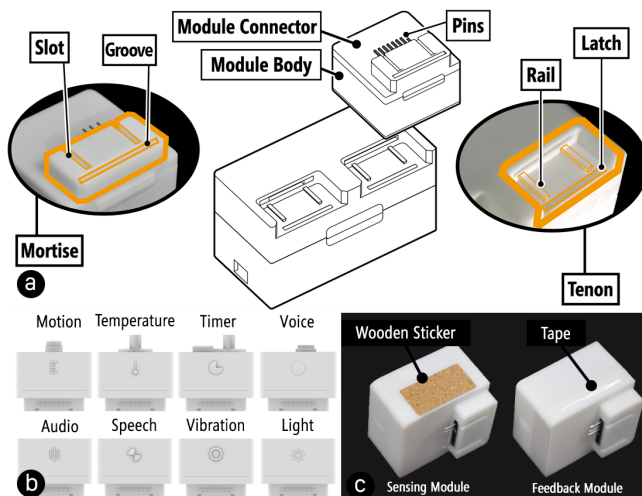
Figure 2: Connector design and tactile labels in A11yBits.
