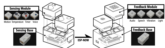
Figure 1: Sensing, Feedback, and Base modules in A11yBits .
