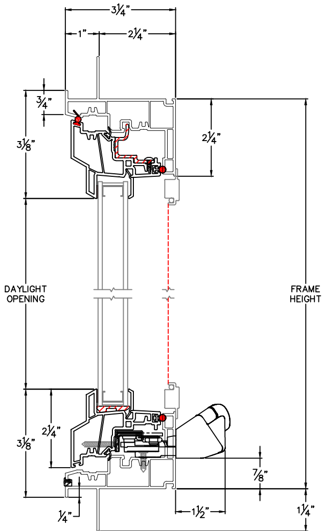
HEAD & SILL
