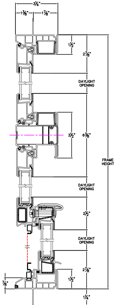
HEAD & SILL
