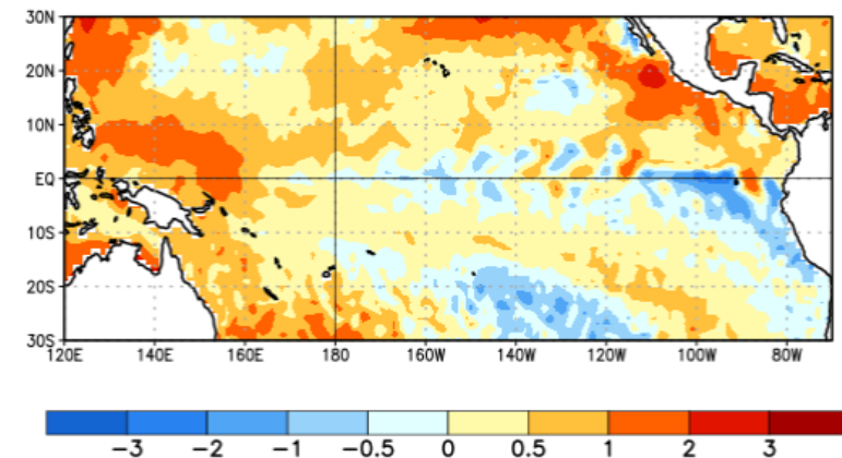
Figure 2: Average sea surface temperature (SST) anomalies ( ^{\circ}\text{C} ) for the week centered on 04 September 2024
