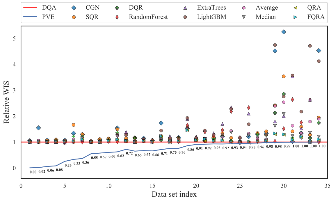
Figure 1: Weighted interval score (WIS), averaged over out-of-sample predictions, for deep quantile aggregation (DQA) and various quantile regression methods. DQA is the most flexible aggregation model of the form (1) that we consider in this paper. The comparison is made over 34 data sets, ordered along the x-axis by proportion of variance explained (PVE), as in (2). The y-axis displays the WIS of each method relative to DQA, so that 1 indicates equal performance to DQA, and a number greater than 1 indicates worse performance than DQA. We can see that DQA performs very well overall, especially for larger PVE values (problems with higher signal-to-noise ratios).
