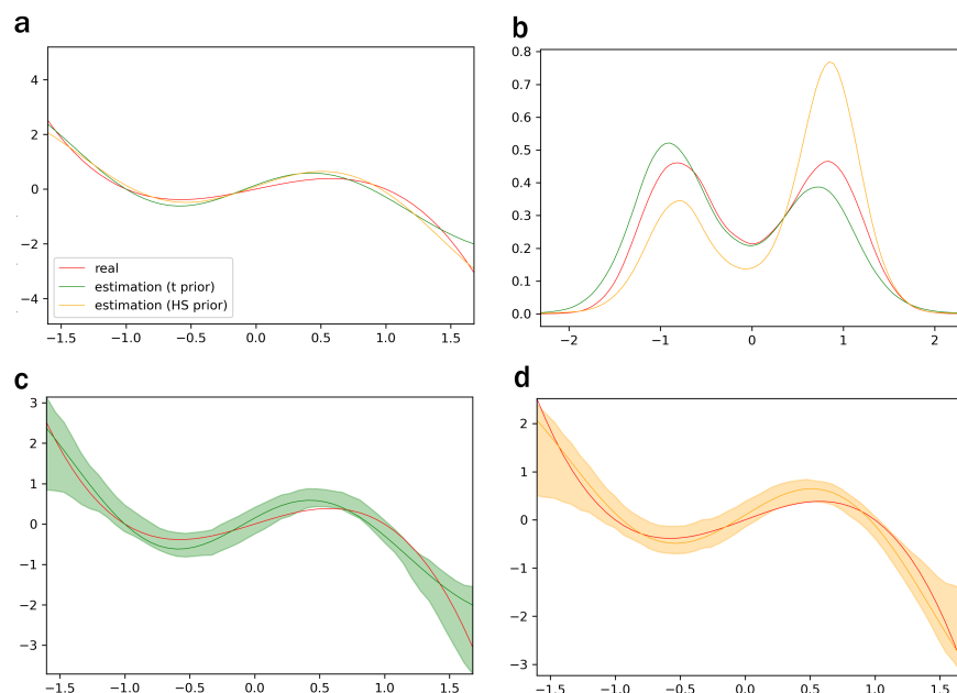
Figure 4: Variant of double-well model ( \zeta = 0.5 ). a: comparison of estimated function \hat{b} with true b . b: comparison of the stationary distributions of the SDE driven by estimated \hat{b} and true b . c, d: estimated function \hat{b} with the shaded areas showing the 95% confidence regions.
