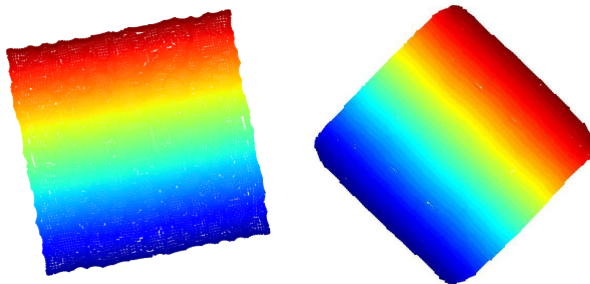
Figure 13: Global embedding of the square grid when the points on the boundary are unknown (left) versus when they are known a priori (right).
