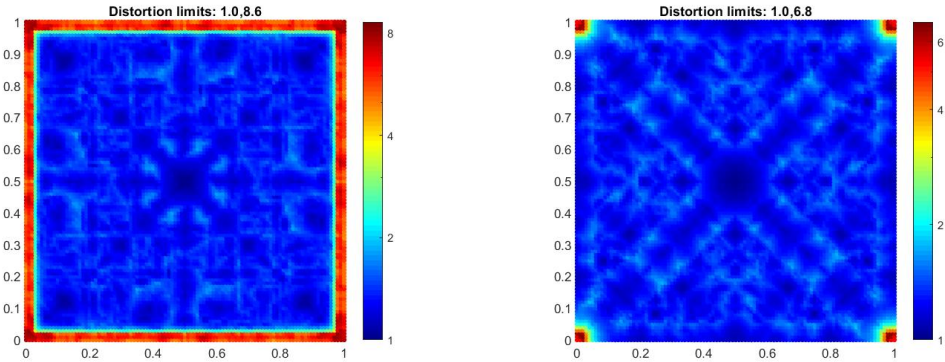
Figure 5: Distortion of the obtained local parameterizations when the points on the boundary are not known (left) versus when they are known a priori (right). Each point x_k is colored by \zeta_{kk} (see Eq. (45)).
