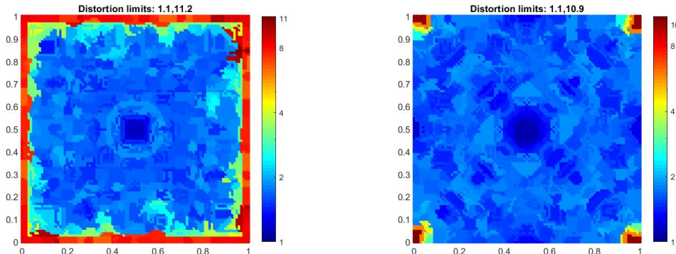
Figure 7: Each point x_k colored by \tilde{\zeta}_{c_k c_k} when the points on the boundary of the square grid are unknown (left) versus when they are known apriori (right).
