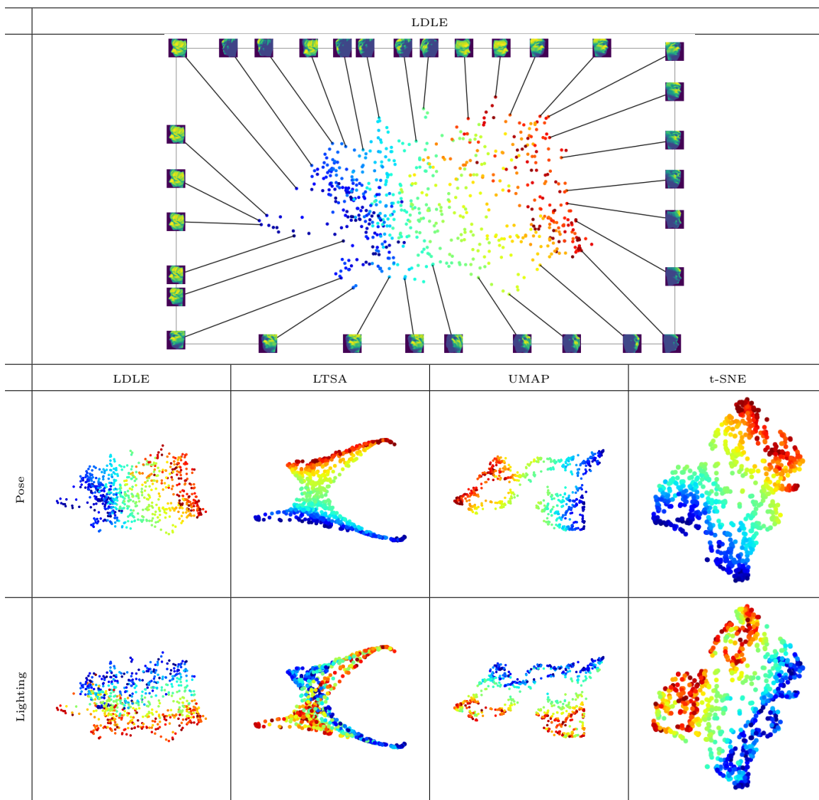
Figure 22: Embedding of the face image data set (Tenenbaum et al., 2000) into \mathbb{R}^2 colored by the pose and lighting conditions (see Section 6.5 for details).
