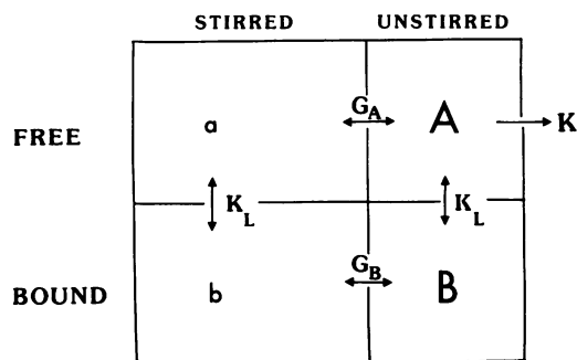
Figure 3. Compartmental model for predicting the effect of an unstirred layer of extracellular fluid. G_A = D_A\phi/\delta , G_B = D_B\phi/\delta .
