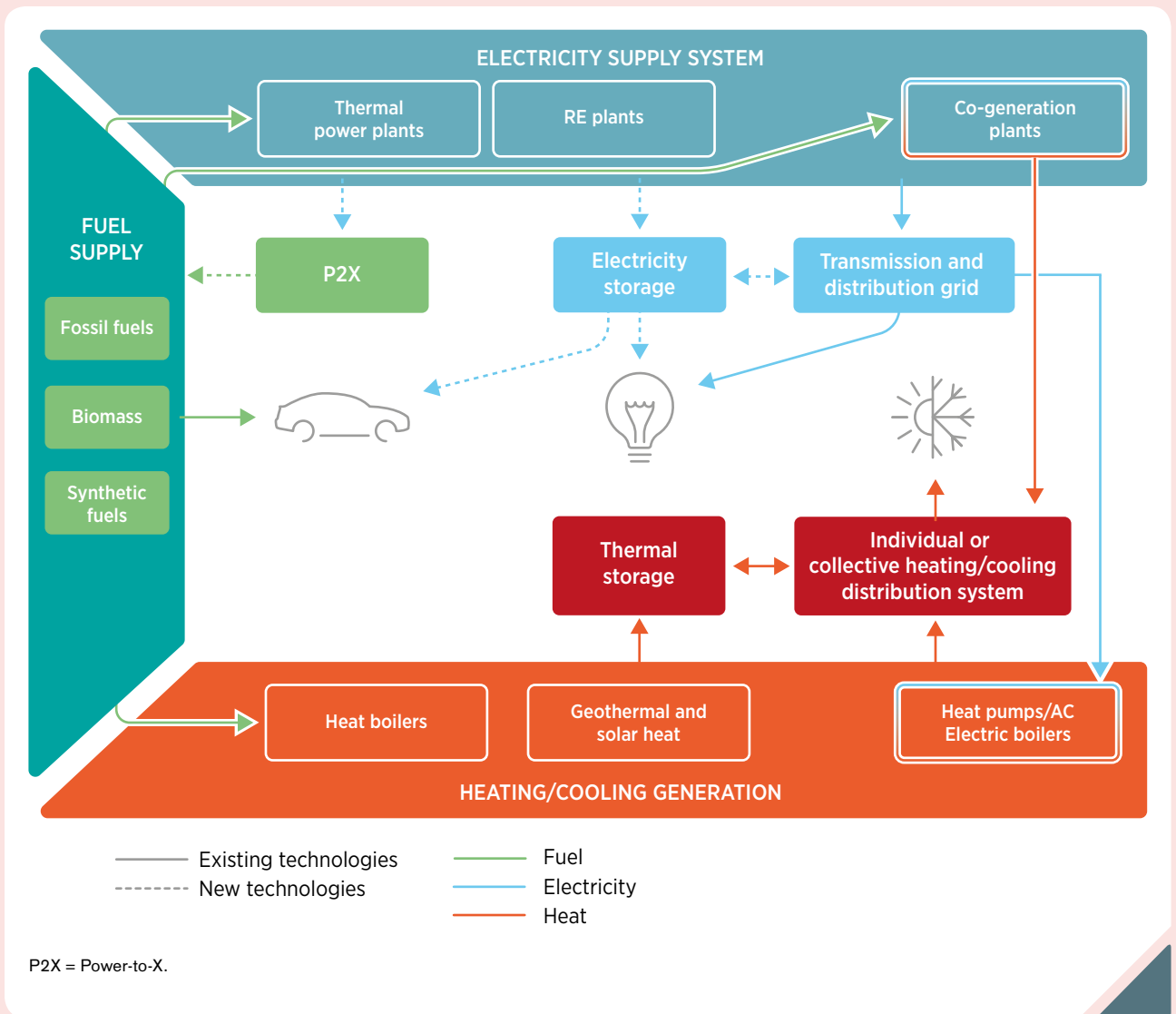
Figure 5.5. Sector coupling
