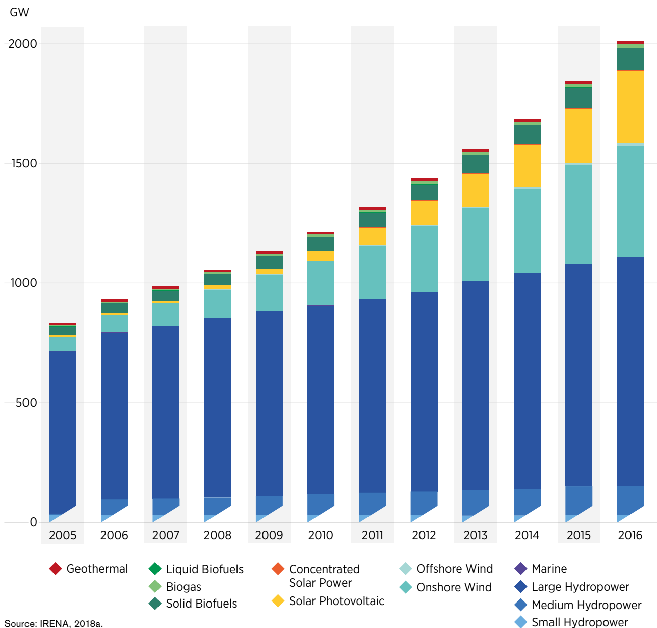
Figure 4.4. Trends in renewable installed capacity, by technology, 2005-16
