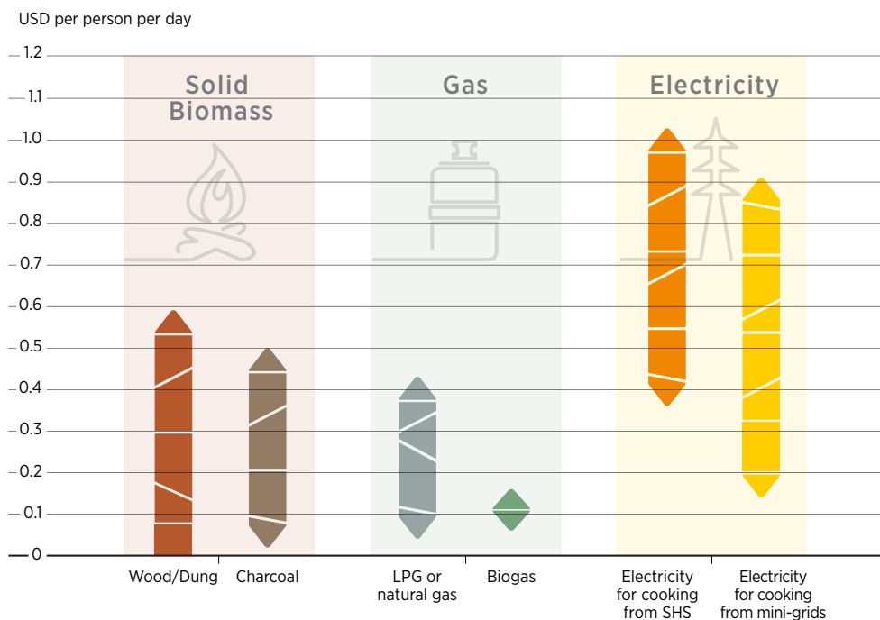
Figure 2.6. Costs of various cooking technologies
