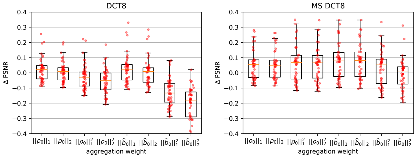
Figure 9: Effect of different aggregation weights on the DCT and MS DCT algorithms (with 8 \times 8 patches) with noise \sigma = 50 and 30 . The PSNR increments (red dots) are computed with respect to the output of the algorithm without aggregation weights for all the images of the training database (Figure 5). The black boxes extend from the lower to upper quartile values of the data and the orange line marks the mean.
