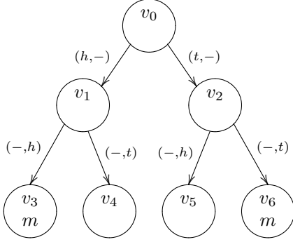
Figure 1: CGS \mathcal{G} for the game of matching pennies
