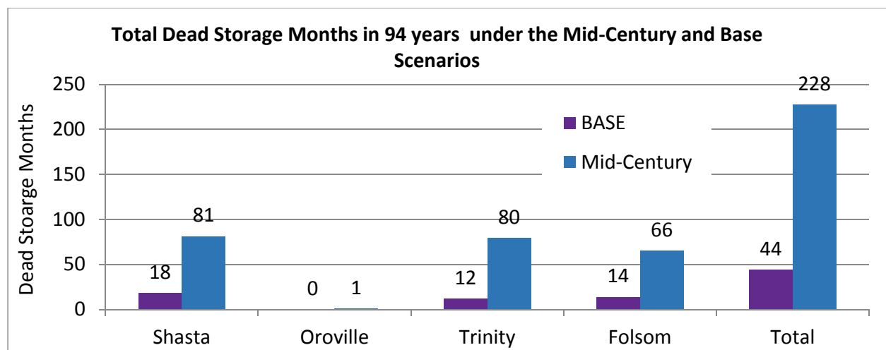
Figure 9: Dead Storage Occurrence for the Base and Mid-Century Scenarios
