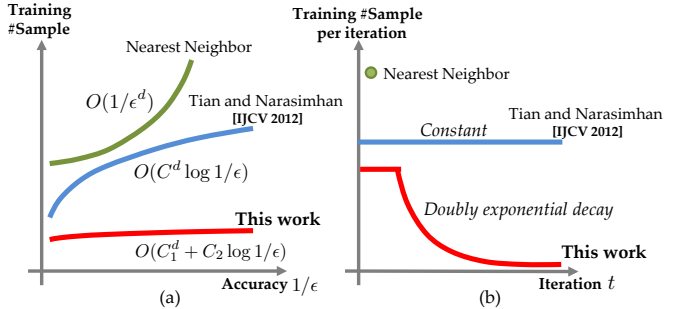
Figure 1. Illustrations of order of training sample complexity required for estimating d dimensional deformation. (a) : To achieve a guaranteed accuracy 1/\epsilon , traditional regression-based approaches (e.g. Nearest Neighbor) require O(1/\epsilon^d) training samples. Data-driven Descent [17] requires O(C^d \log 1/\epsilon) , decoupling the dimensionality from the accuracy. Our hierarchical framework for deformation estimation achieves O(C_1^d + C_2 \log 1/\epsilon) with constant C_1 much smaller than C and C_2 independent of dimensionality. (b) Sample complexity per iteration. A constant number of samples per iteration is needed in [17]. The number of samples needed is a constant for the first few iterations, and then decays double exponentially for our algorithm.
