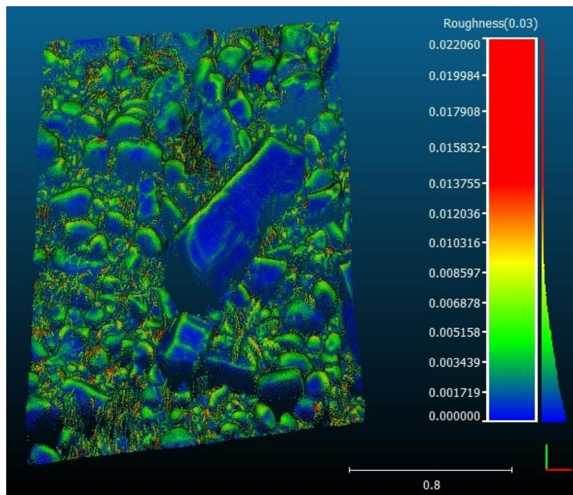
Roughness output
