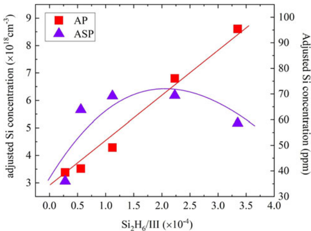
Fig. 8. Si concentration of the \text{Al}_x\text{Ga}_{1-x}\text{N}:\text{Si} -doped layer as a function of disilane to group III ratio, as evaluated by WDX. The solid lines provide guides to the eye.
