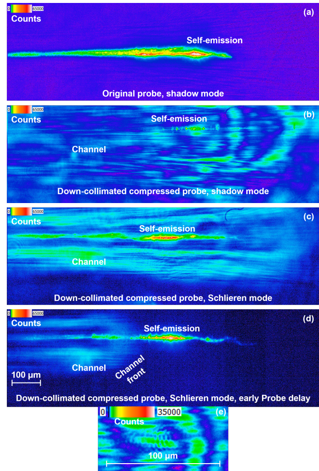
Figure 6. (a-d) Representative examples of images produced by the original and down-collimated compressed probe, magnification M = 10.2 , frame size 1920 \times 600 pix = 1.1 \times 0.34 mm. The scale bar shown in (d) is common for (a-d). (a) Original probe, the shadow mode. (b) Down-collimated compressed probe, the shadow mode. (c) Down-collimated compressed probe, the Schlieren mode. (d) Down-collimated compressed probe, the Schlieren mode at an early probe delay. (e) A representative example of fine fringes observed by the compressed probe; note the difference in scale compared to (a-d).
