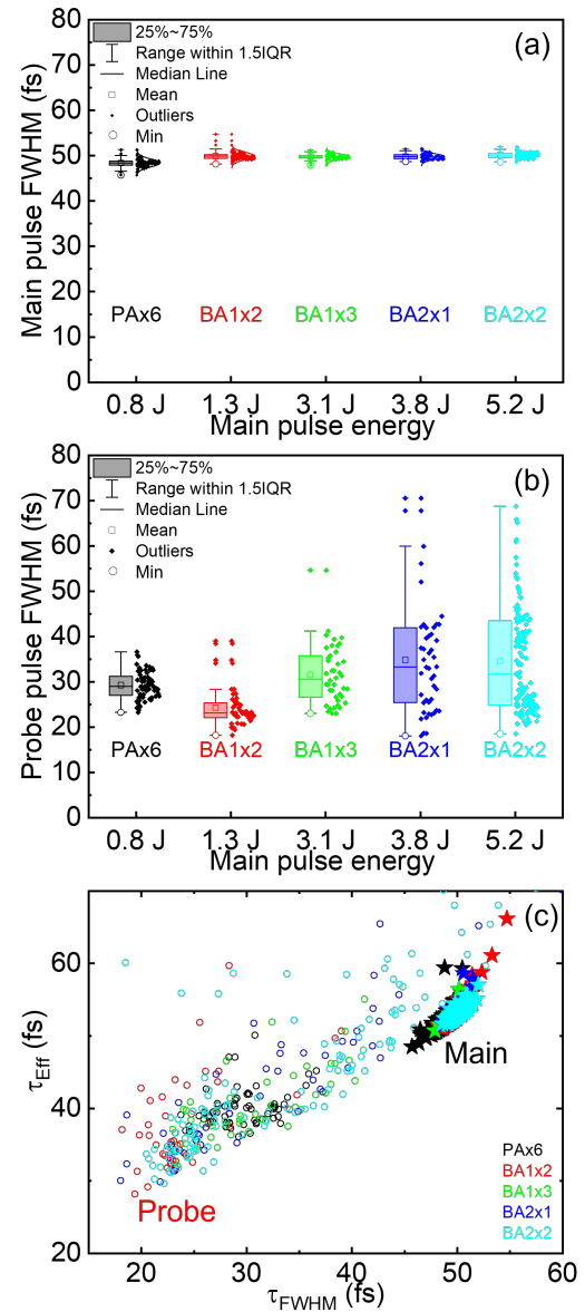
Figure 3. On-shot main and probe pulse measurements during one experimental day in several laser modes. The box-and-whisker plots of the main pulse (a) and probe pulse (b) FWHM durations vs. laser mode and main pulse energy. The colored bars represent the 25%-75% ranges, the error bars are the 1.5 interquartile ranges, the horizontal lines are the medians, while the squares, dots, and circles are the means, outliers, and minima, respectively. The dots on the right from the boxes-and-whiskers are the individual shots forming the corresponding histograms. (c) Main (stars) and probe (rings) pulse on the [FWHM, effective pulse width] plane; each point is an individual shot. Color encodes the laser mode.
