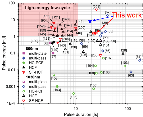
Figure 7. Comparison with other works. Our average BA1x2 data and best BA2x1 data are shown with the red and blue stars, respectively. The figure with other data is reprinted with permission from [21].
