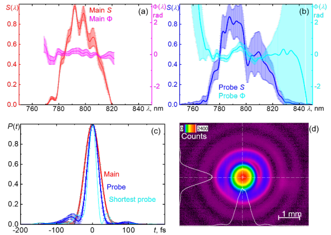
Figure 2. Main and probe pulses before the experiment. (a, b, c) Power Amplifier (PA) mode, \sim 1000 -shot average for the main and probe pulses, the error bars are standard deviations of shot-to-shot variations. (a) Red is the main pulse spectra, magenta is the main pulse spectral phase. (b) Blue is the probe pulse spectra, cyan is probe pulse spectral phase. (c) Red and blue, the main and probe pulse shapes, cyan: the shortest probe pulse. (d) Down-collimated probe beam spatial profile measured before the fused silica plates by using a low-power infrared laser diode alignment beam.
