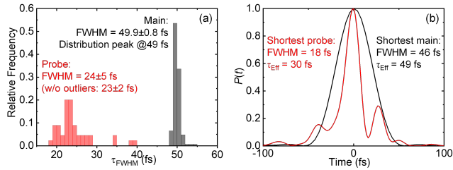
Figure 4. Stability of the probe pulse compression and the shortest measured pulses. (a) FWHM histograms for the BA1x2 mode, which provides the optimum average compression. (b) Shortest main and probe pulses, the latter was obtained in the BA2x1 laser shot with the main pulse energy of 4 J and probe pulse energy of \sim 5.8 mJ.
