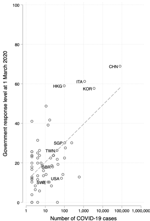
Figure 4: Response-Risk Ratio
