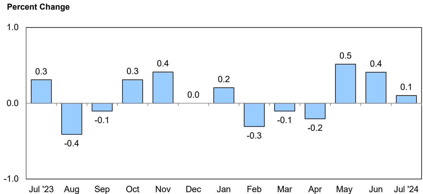
Chart 2: Over-the-month percent change in real average hourly earnings for production and nonsupervisory employees, seasonally adjusted, July 2023–July 2024
