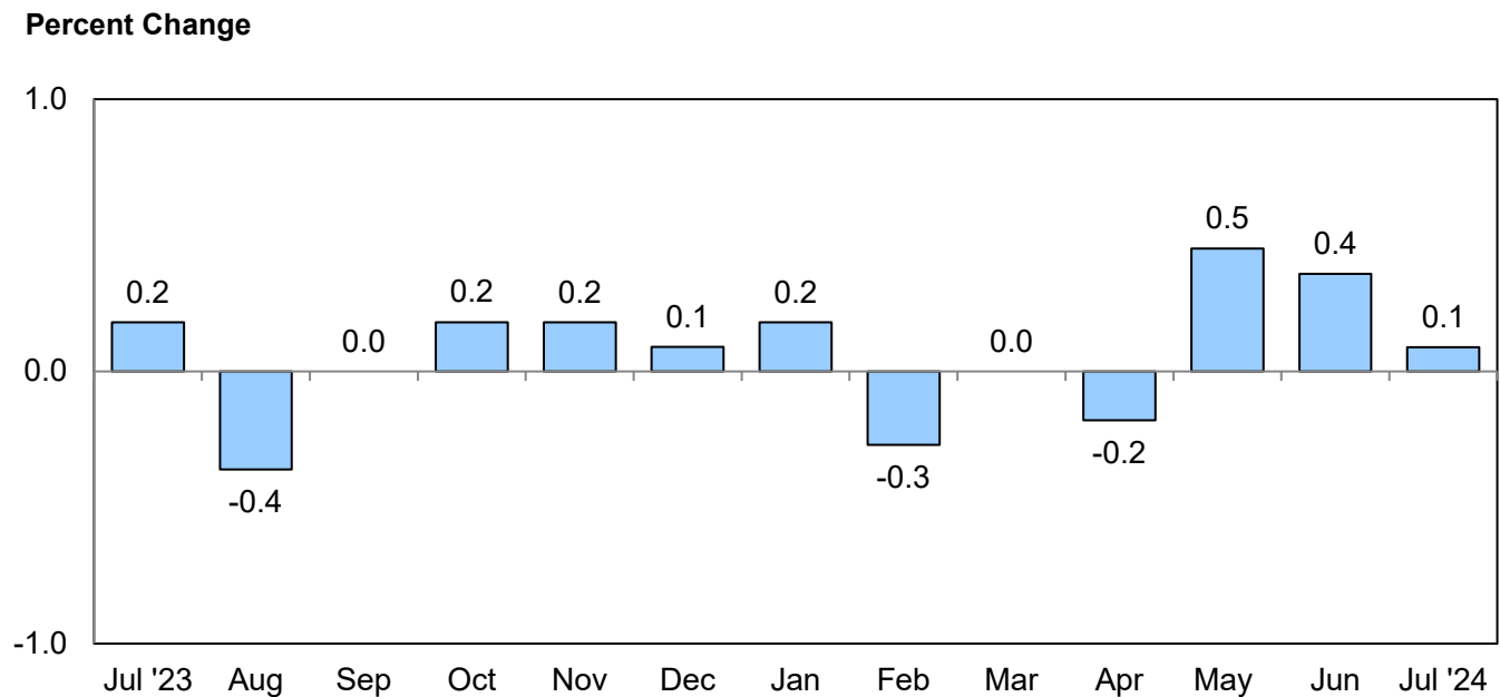
Chart 1: Over-the-month percent change in real average hourly earnings for all employees, seasonally adjusted, July 2023–July 2024
