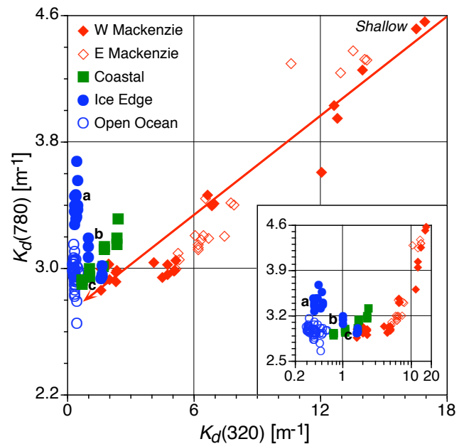
Fig. 7. A plot of K_d(320) versus K_d(780) for the Malina sampling, which was centered around the Mackenzie River outflow, using the same symbols as Fig. 1. The sampling included the following water masses: the open ocean (open blue circles), the western branch of the Mackenzie River (solid red diamonds), the eastern branch of the Mackenzie River (open red diamonds), coastal waters (green squares) and the ice edge (solid blue circles). The latter are further distinguished by the influence of the Mackenzie River plume: (a) no influence; (b) some influence; and (c) the most influence. The overlaid red arrow shows a progression in water properties from shallow waters (top right) to deep waters (bottom left). The inset panel shows the same data with a logarithmic x-axis to improve the clarity of the data with low K_d(320) values.
