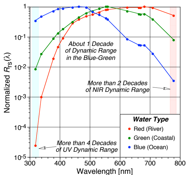
Fig. 2. Averaged Malina R_{rs}(\lambda) = L_W(\lambda)/E_d(0^+, \lambda) spectra, normalized by the peak value of the spectrum. The spectra are separated into three groups based on the peak wavelength domain (blue, green, and red) and classified as river, coastal, or ocean based on the preponderance of the sampling locations.
