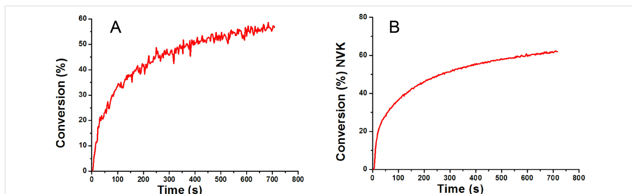
Figure 10: (A) Photopolymerization profile of EPOX; photoinitiating system: \text{Ir}(\text{piq})_2(\text{tmd})/\text{Ph}_2\text{I}^+/\text{NVK} (1%/2%/3%); laser diode at 532 nm exposure ( \sim 100 mW/cm ^2 ); under air. (B) Conversion profile for the NVK double bond in the course of the polymerization.
