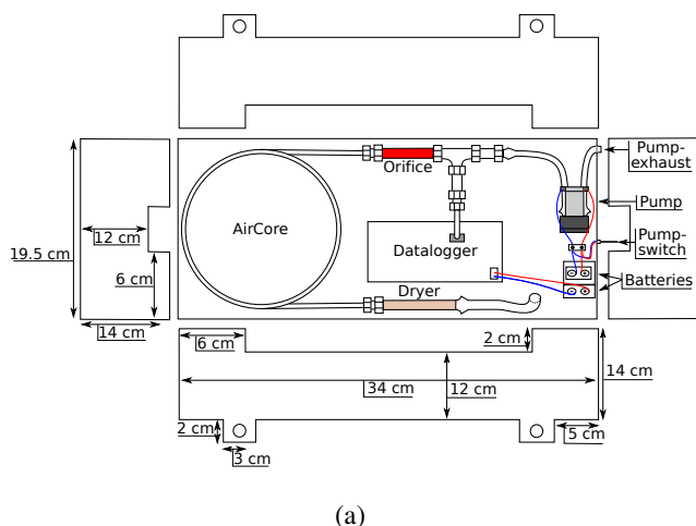
Figure 1. (a) Schematic design of the UAV AirCore system. (b) Image of the UAV AirCore system.
