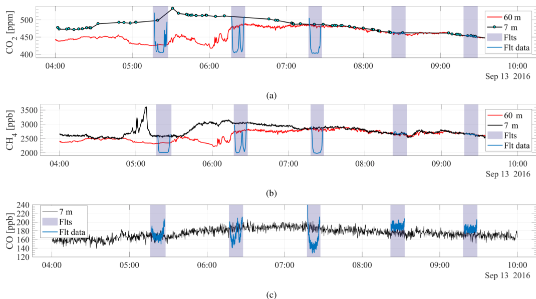
Figure 8. The continuous CO 2 (a), CH 4 (b), and CO (c) measurements from the atmospheric tower at 7 m (black) and 60 m (red), along with the mole fractions measured with the active AirCore (blue). The highlighted areas indicate the time span for each of the flights, approximately spaced 1 h apart. The altitude covered during the flights was 485, 301, 478, and 23 m for flight nos. 1, 2, 3, and 4, respectively, transecting both the 7 and 60 m altitudes. Flight no. 5 hovered at 60 m close to the 60 m tower inlet.
