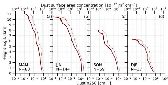
Figure 16. Same as Fig. 12 except for the seasonal mean dust particle number concentration n_{250,d} (considering particles with radius > 250 \text{ nm} ) and dust surface area concentration.
