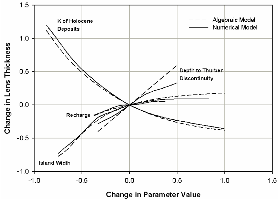
Figure 49. Comparison between the sensitivity of the parameters in the algebraic and numerical models. Only the derivative of the depth to Thurber Discontinuity parameter shows a deviation from the numerical results.
