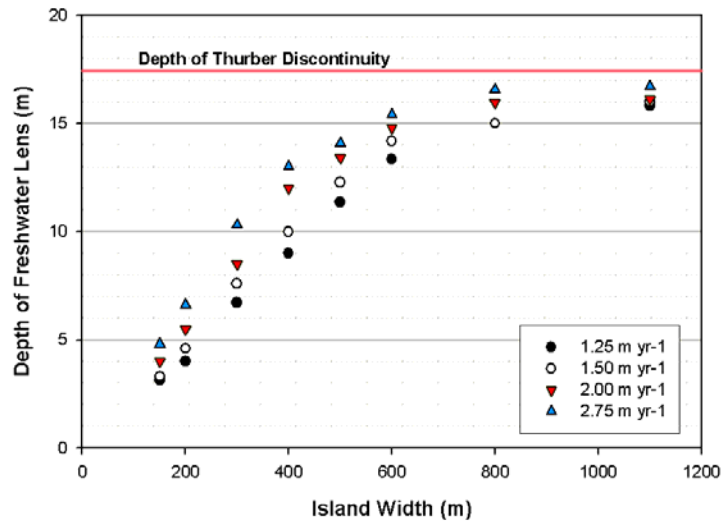
Figure 17. Results from the rainfall experiment, showing the increase of lens thickness with increasing rainfall rates
