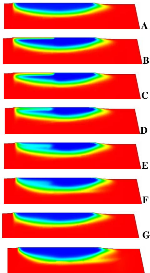
Figure 39. Contamination and recovery of the freshwater lens from a 48-hour washover event, at (A) initial conditions, (B) 16 hours, (C) 48 hours, (D) 1 month, (E) 2 months, (F) 4 months, (G) 1 year, (H) and 1 ½ years. The portion of the lens on the ocean side, underneath the reef flat plate, is protected from contamination.
