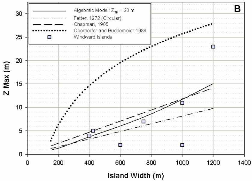
Figure 52. Comparison of observed lens depths on atoll islands, results from the algebraic model, the analytical modes proposed by Fetter (1972) and Chapman (1985) for oceanic islands, and the empirical model proposed by Oberdorfer and Buddemeier (1988), for (A) leeward islands, using a K factor corresponding to a hydraulic conductivity of 50 m day -1 , and (B) windward islands, using 400 m day -1 .
