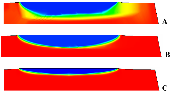
Figure 19 Lens geometry for hydraulic conductivity values of (A) 25 \text{ m day}^{-1} , (B) 100 \text{ m day}^{-1} , and (C) 400 \text{ m day}^{-1}
