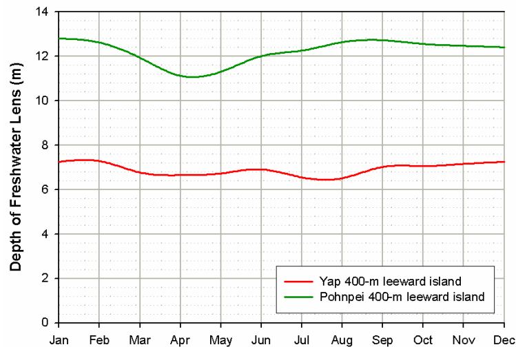
Figure 34. Comparison of lens behavior between leeward islands located in the Western Caroline region (Yap) and the Eastern Caroline region (Pohnpei).
