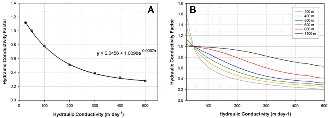
Figure 46. (A) Trend between the hydraulic conductivity of the Holocene sediments and the associated hydraulic conductivity factor, for an island width of 500 m, and (B) for each island width
