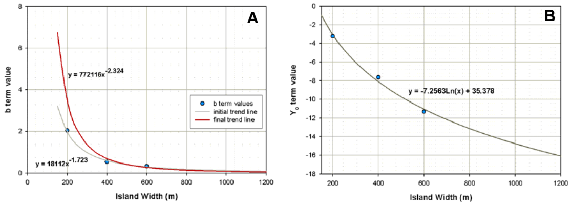
Figure 44. Curve-fitting to produce trends of (A) B parameter and (B) Y parameter
