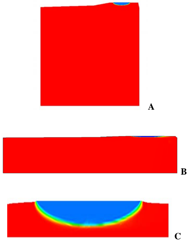
Figure 14. Typical freshwater lens delineation, (A) with vertical exaggeration and (B) without vertical exaggeration, and (C) an enlarged view of the island subsurface
