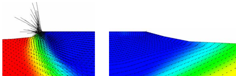
Figure 27. The direction and magnitude of the groundwater flow on (a) the lagoon side, where no reef flat plate exists, and (b) the ocean side.
