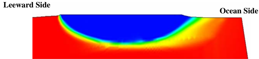
Figure 26. The freshwater lens configuration when a reef flat plate is present on the ocean side, for a 400 m wide island. Notice the thickness of the transition zone on the ocean side, as compared to the leeward side.
