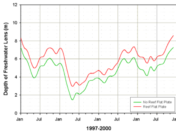
Figure 32. Effect of including the reef flat plate on the freshwater lens
