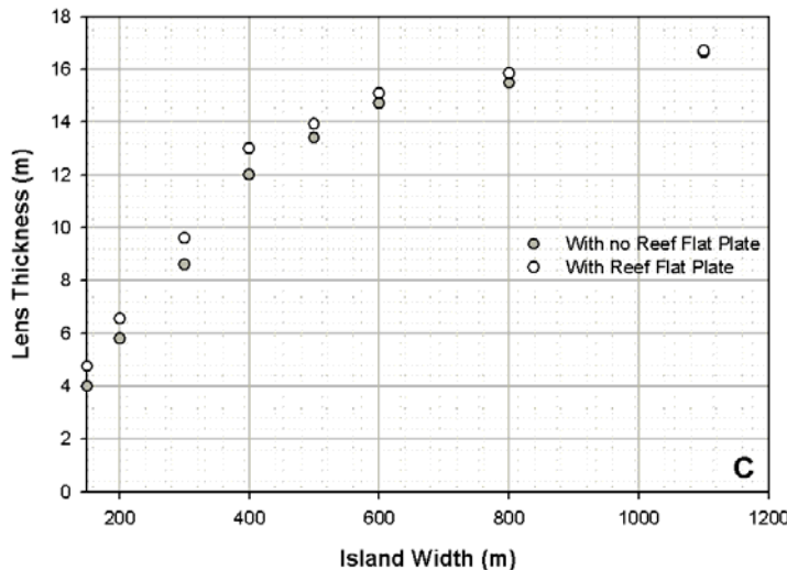
Figure 25. The lens thickness as the island width is varied, for simulations with and without a reef flat plate. Notice that the difference between the two simulations decreases as the island width
