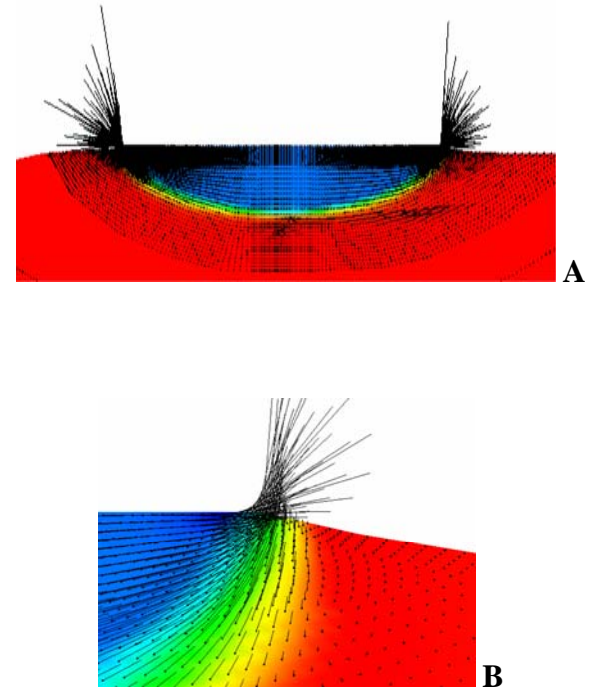
Figure 15. (A) View of velocity vectors, with the black circles as the tail, of the groundwater flow, and (B) Enlarged view of the direction and magnitude of groundwater flow at the coastline.
