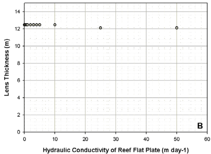
Figure 29. The thickness of the lens as the reef flat plate hydraulic conductivity is varied. The thickness is minimally affected.
