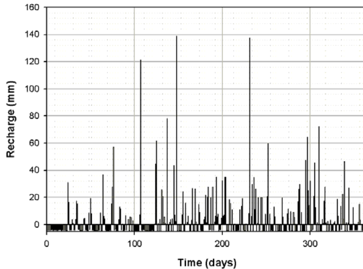
Figure 31. Daily recharge for Yap, 2000
