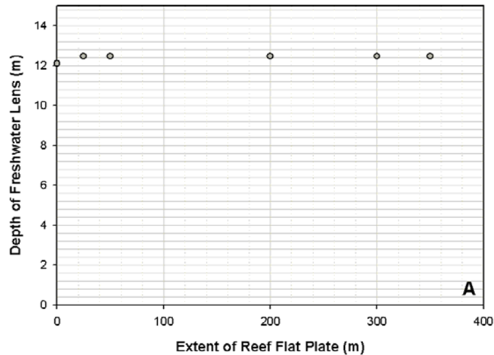
Figure 28. The thickness of the lens as the reef flat plate is extended to various distances across the atoll islands. The thickness is minimally affected.
