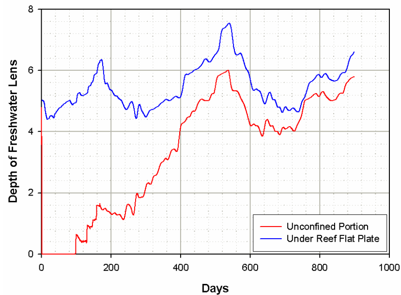
Figure 40. Recovery of the freshwater lens after a two-day washover event, (blue) underneath the reef flat plate, on the ocean side, and (red) in the unconfined region on the leeward side
