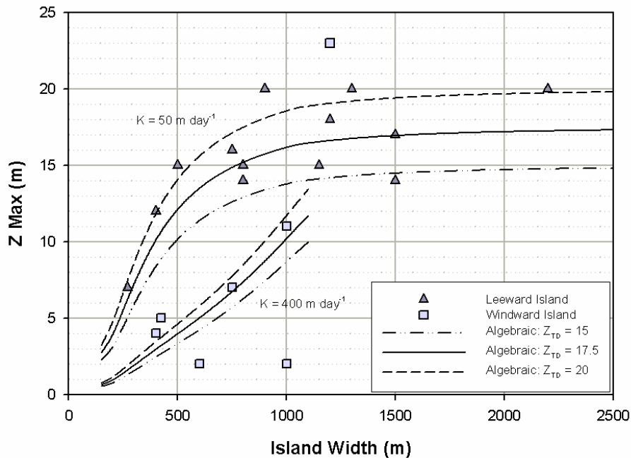
Figure 51. Comparison between observed lens maximum depths and results from the algebraic model. One curves used Thurber Discontinuity depths of 15, 17.5, and 20 m, which are typical depths. The curves passing through the leeward islands were created using a K factor corresponding to a hydraulic conductivity of 50 m day -1 , while the curves passing through the windward islands used 400 m day -1 .
