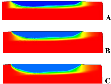
Figure 23. Lens geometries for a Thurber Discontinuity depth of (a) 10 m, (b) 14 m, and (c) 18 m
