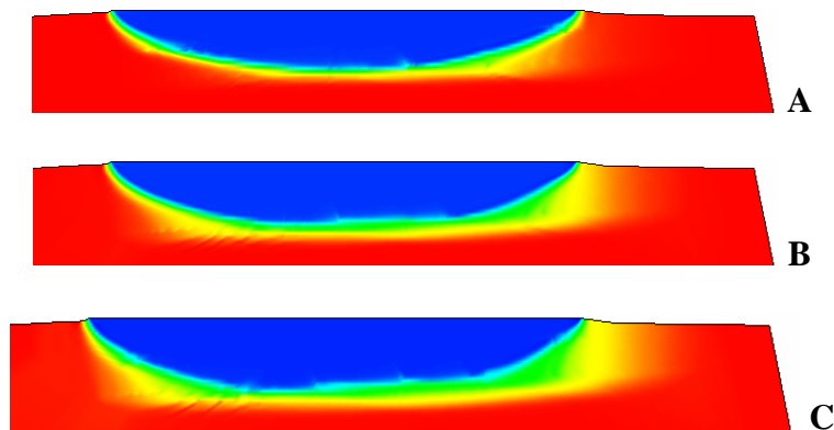
Figure 16. Lens geometry for a 600-m island for recharges rates of (A) 1.25 m yr -1 , (B) 2 m yr -1 , and (C) 2.75 m yr -1
