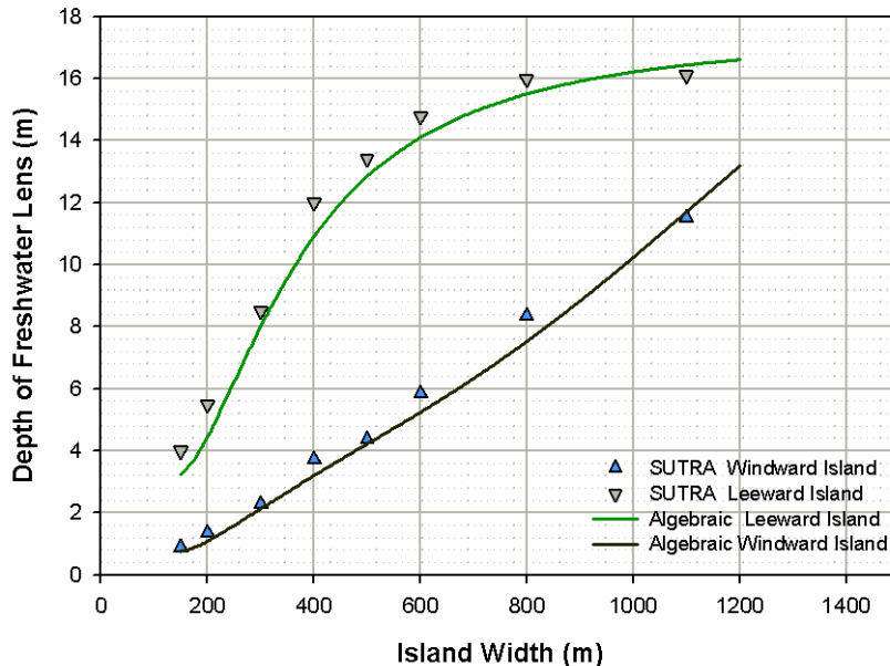
Figure 50. Comparison of SUTRA simulation results with the Algebraic model results. The SUTRA Leeward island simulations used a hydraulic conductivity value of 50 m day -1 , and the algebraic model used a K factor for a hydraulic conductivity value of 50 m day -1 . Similarly, the SUTRA Windward island simulations used a K hydraulic conductivity value of 400 m day -1 , and the algebraic model used K factors corresponding to a hydraulic conductivity value of 400 m day -1 .
