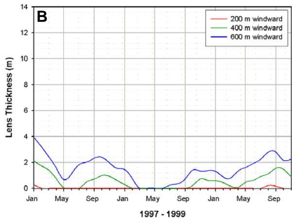
Figure 36. Thickness of the lens as it responds to an El Niño event, for (A) leeward islands and (B) windward islands located in the Western Caroline Islands. The windward islands, with a much higher hydraulic conductivity than leeward islands, have much thinner lenses.
