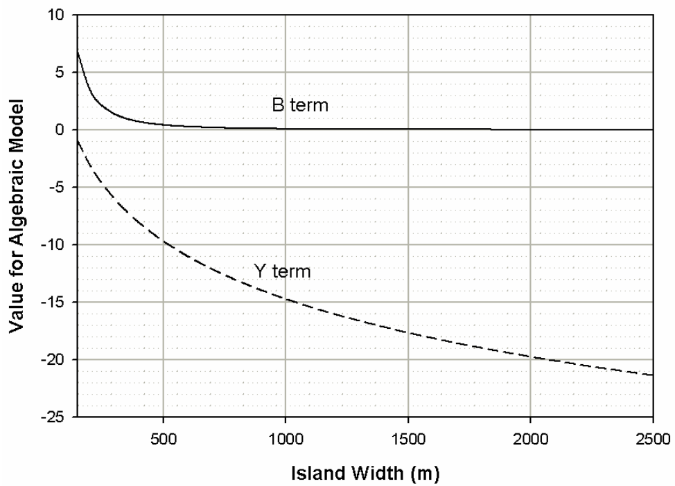
Figure 45. Curves for B and Y parameters of the Algebraic Model
