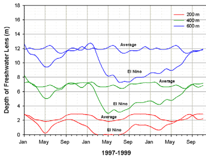
Figure 38. Comparison of the lens depth through time for average seasonal weather patterns and an El Niño event, in the Western Caroline region, for island widths of 200, 400, and 600 m. The upper and lower curves for each island width correspond to average and El Niño conditions, respectively.
