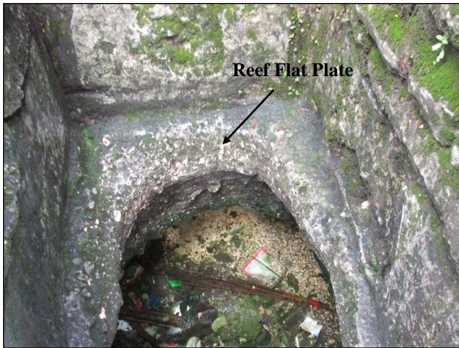
Figure 9. (A) Well on Mogmog Island, Ulithi Atoll showing reef flat plate, and (B) Close-up view of reef flat plate. The reef flat plate, located at mean sea level and extending across much of the island, is a confining layer to the freshwater. Residents of atoll islands are thus required to punch through the plate to reach the freshwater if they dig wells on the ocean side of the island.
