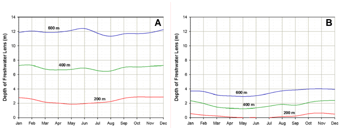
Figure 33. Thickness of the lens as it responds to regular seasonal rainfall variation, for (A) leeward islands and (B) windward islands located in the Western Caroline Islands. The windward islands, with a much higher hydraulic conductivity than leeward islands, have much thinner lenses. The lens of the 200 m wide windward island is altogether depleted during the dry summer months.
