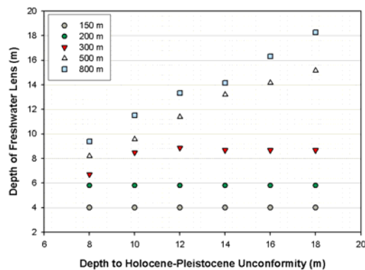
Figure 24. Results from the Thurber Discontinuity experiment, showing the lens thickness vs. the depth to the unconformity for 5 different island widths. Notice that the smaller islands are not affected by the unconformity.
