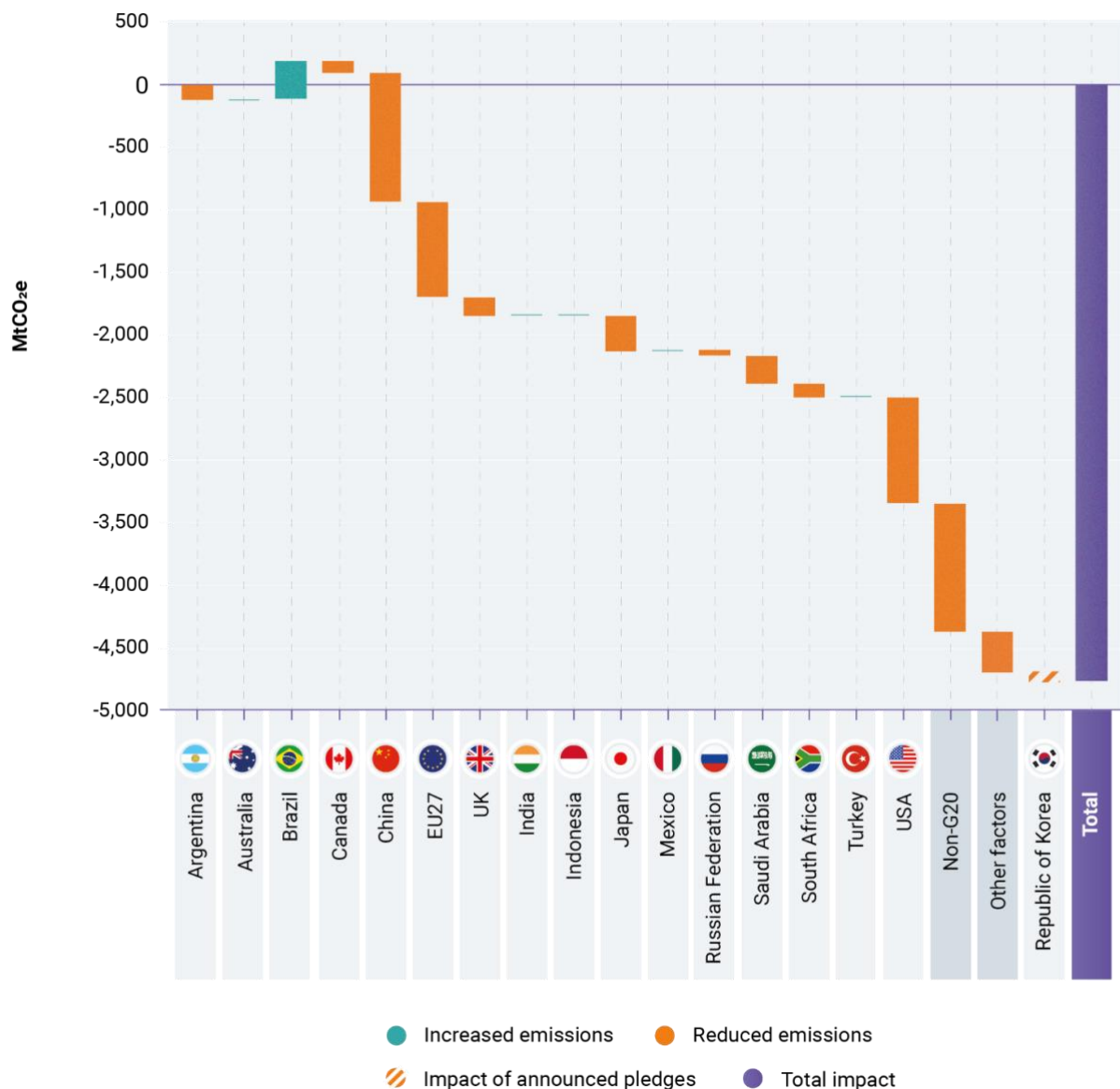
Figure 1. Preliminary update of the impact of unconditional 2030 pledges (NDCs and other pledges) on 2030 global emissions compared with the first round of nationally determined contributions.
