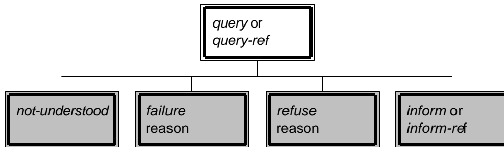
Figure 4 — FIPA-Query Protocol
