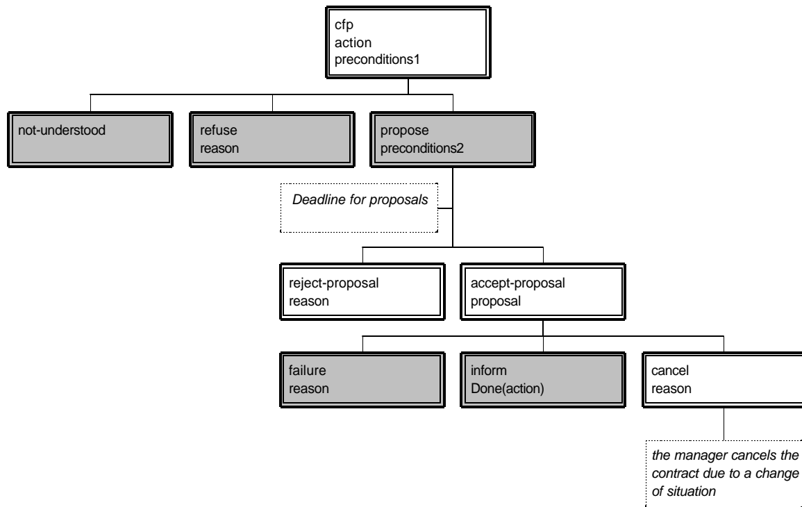
Figure 6 — FIPA-Contract-Net
