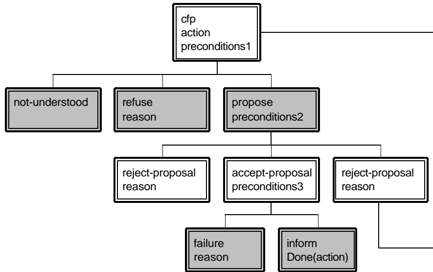
Figure 7 — FIPA-iterated-contract-net protocol
