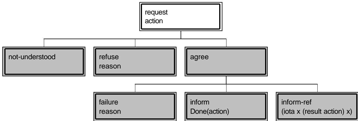
Figure 3 — FIPA-Request Protocol
