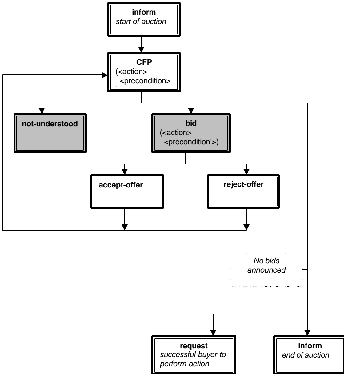
Figure 8 — FIPA-auction-english protocol
