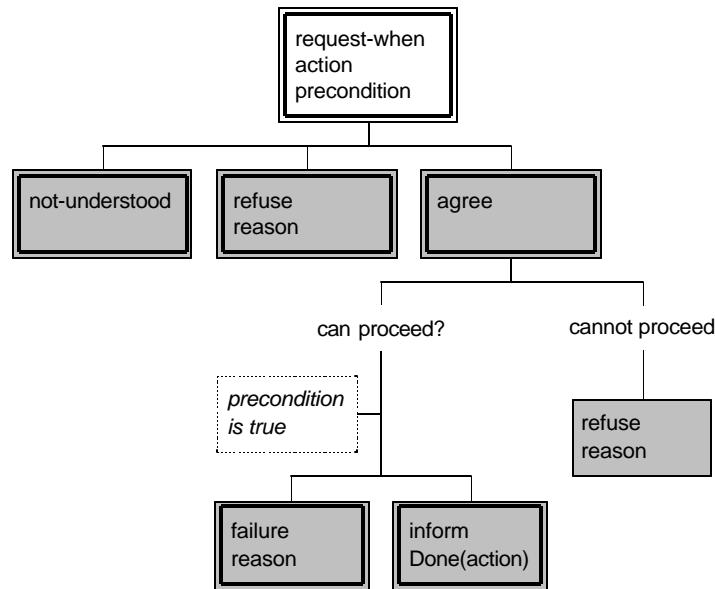
Figure 5 — FIPA-request-when protocol
