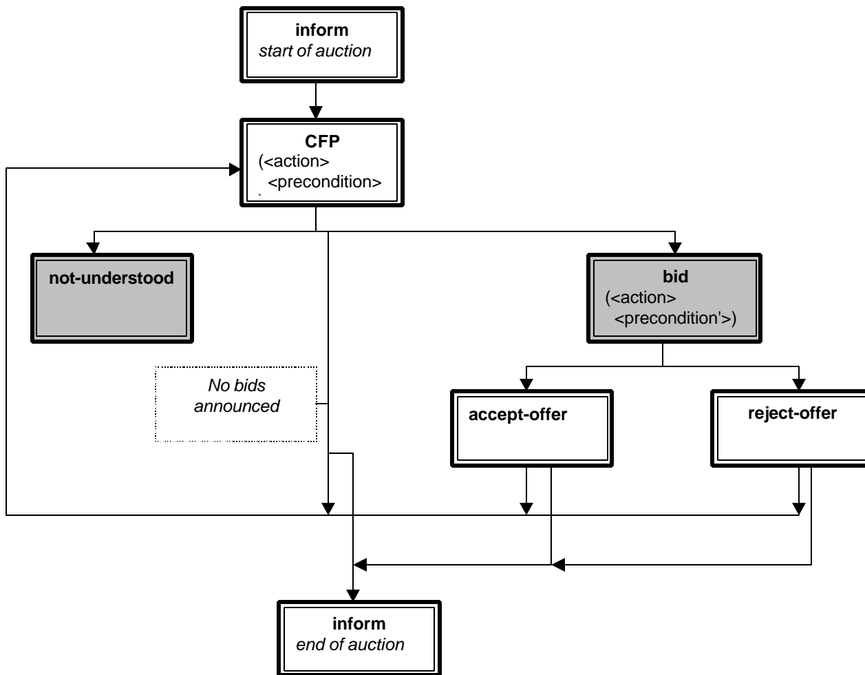
Figure 9 — FIPA-auction-dutch protocol
