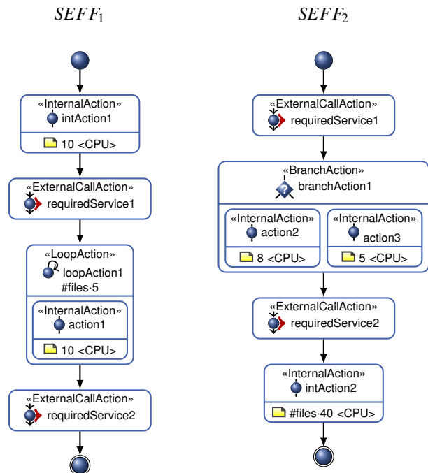
Figure 4. Refinement Example
