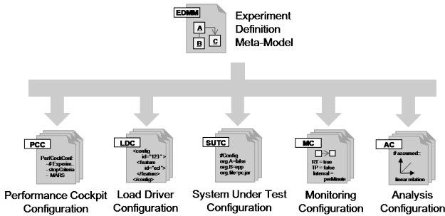
Fig. 3. ExperimentDefinitionMetaModel
