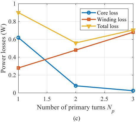
Fig. 18. Calculated power losses of planar transformers with different winding arrangements and different numbers of primary turns N_p : (a) non-interleaving winding arrangements: P-S for N_p = 1 , P-P-S-S for N_p = 2 , P-P-P-S-S-S for N_p = 3 , (b) interleaving winding arrangement: P-S for N_p = 1 , P-S-P-S for N_p = 2 , P-S-P-S-P-S for N_p = 3 , (c) 0.5P-S-0.5P for N_p = 1 , 0.5P-S-P-S-0.5P for N_p = 2 , 0.5P-S-P-S-P-S-0.5P for N_p = 3 .
