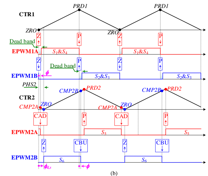
Fig. 23. Modulation waveforms based on TMS320F28075 DSP (a) \phi > \phi_{d,s} , (b) \phi \leq \phi_{d,s} . PRD1 and PRD2 represent the period registers of the two ePWM modules (ePWM1 and ePWM2), PHS2 is the phase register of ePWM2, CMP2A and CMP2B are the counter-compare A and B registers of ePWM2. CAU indicates the event when the counter CTR2 equals the active CMP2A register and CTR2 is incrementing. CAD indicates the event when the counter CTR2 equals the active CMP2A register and CTR2 is decrementing. CBU indicates the event when the counter CTR2 equals the active CMP2B register and CTR2 is incrementing. CBD indicates the event when the counter CTR2 equals the active CMP2B register and CTR2 is decrementing. Z and P represents the events when the counter equals zero and the period, respectively.
