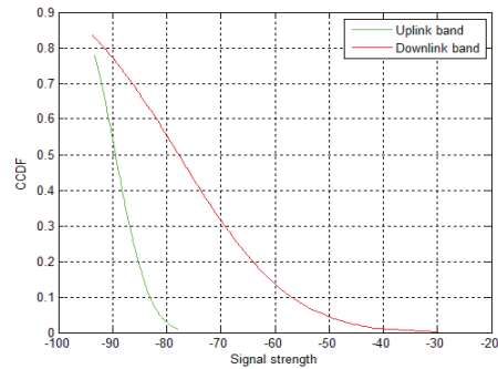
Figure 11. CCDF of GSM 1800 band for scenario 4.
