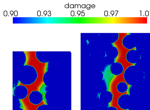
Figure 15: Bulk versus crack homogenization for random microstructure under shear loading.
