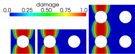
Figure 6: Damage patterns of three samples under horizontal tensile loading.
