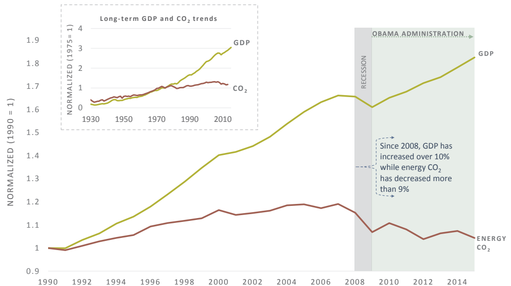
FIGURE E10: U.S. ENERGY CO 2 EMISSIONS AND GROSS DOMESTIC PRODUCT
