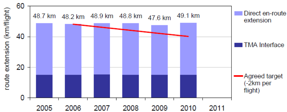
Figure 8 Horizontal flight extension , targets and TMA Interface
