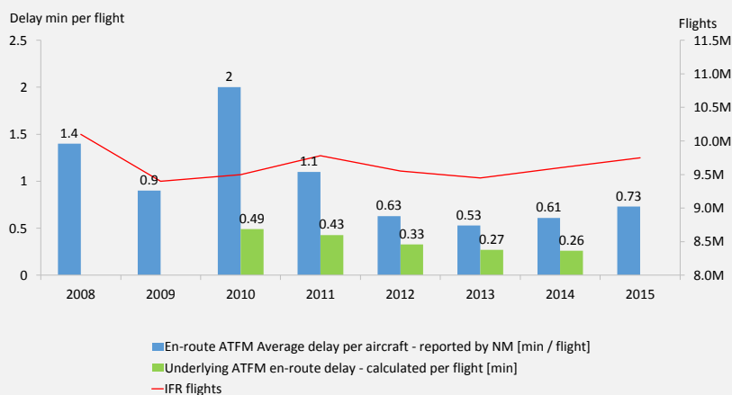
Figure 3 Study team estimate of underlying delay
