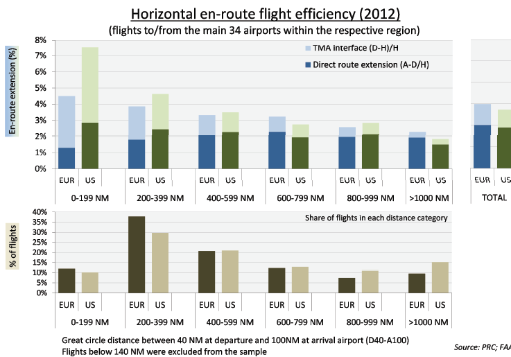
Figure 9 Horizontal en-route flight efficiency
